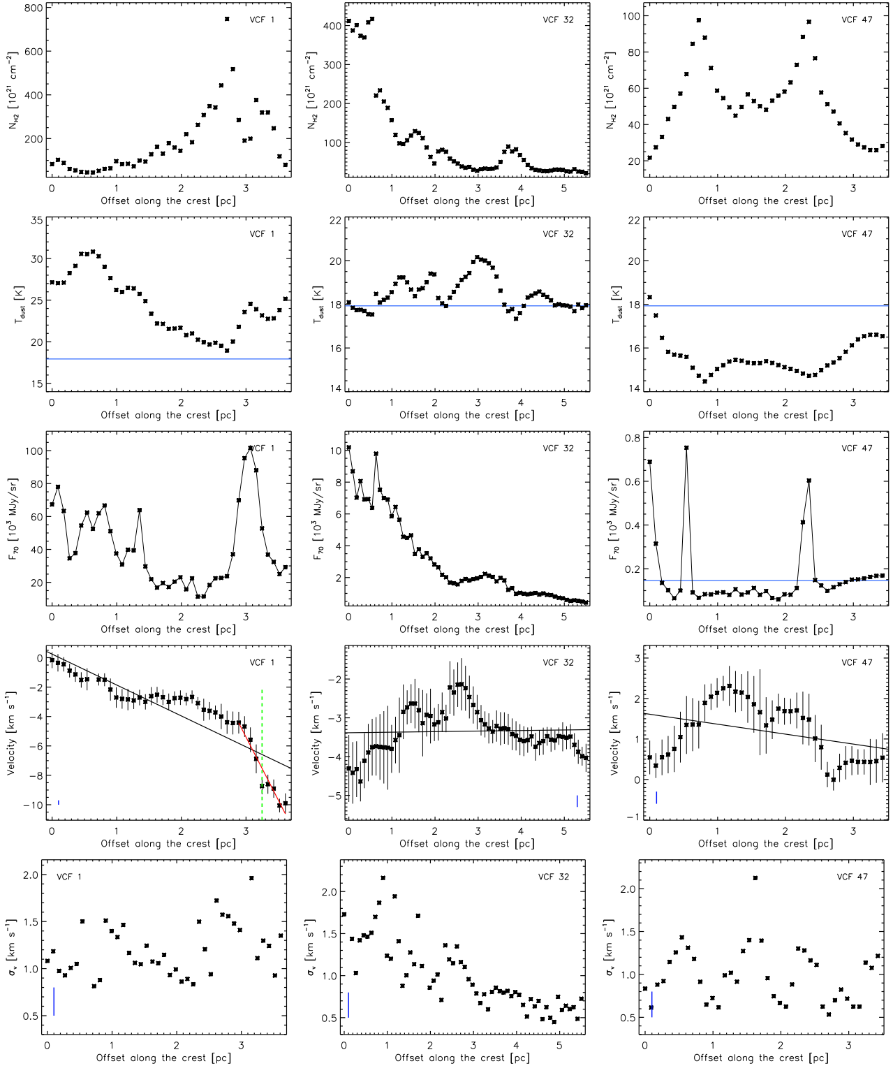
Fig. 10. Properties along VCF crests 1, 32, and 47 (from left to right). The zero offsets correspond to the most southwestern end of the crests (as seen on Fig. 6). Rows from top to bottom: (1) column density derived from Herschel data. (2) LOS averaged dust temperature derived from Herschel data. The horizontal blue lines indicate the mean background temperature around the VFCs of \sim 17.9 \pm 0.2 K. (3) PACS 70 \mu\text{m} flux. The horizontal blue line indicates the mean background emission of \sim 146 \pm 23 MJy sr ^{-1} . (4) Velocity. The black vertical lines on each data point show the velocity dispersion (same as the values shown in row 5). The black lines show a linear fit to these data points. The velocity resolution of 0.3 km s ^{-1} is indicated by the vertical blue lines. For VCF 1, a linear fit to the velocity > 2.8 km s ^{-1} over a length of 0.7 pc is indicated in red and corresponds to the crest crossing the young star cluster identified as source I (see, e.g., Persi & Tapia 2008). The position of source I is indicated with the vertical dashed green line (see also the green arrow in Fig. 6). (5) Velocity dispersion. The velocity resolution of 0.3 km s ^{-1} is indicated by the vertical blue lines.
