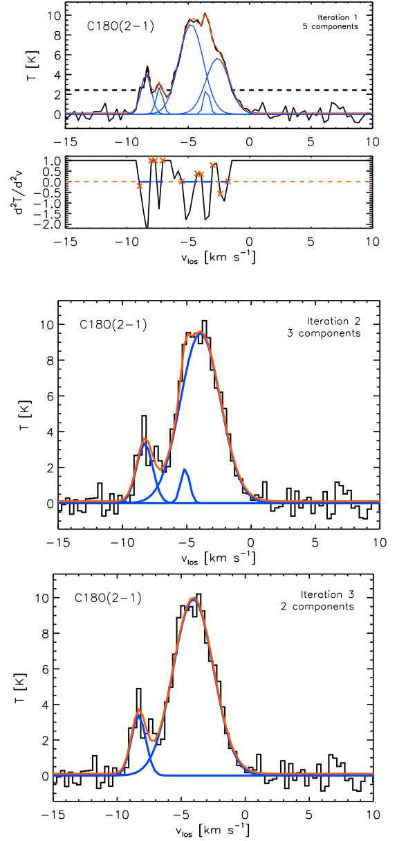
Fig. B.1: Example of an observed spectrum and the different steps of the n -Gaussian fitting procedure. Top : Observed C 18 O(2–1) spectra toward a position in the center of the map (top). The blue and red curves show the five individual Gaussian functions and the sum of all the fitted Gaussians, respectively. The dotted line shows the intensity threshold corresponding to S/N = 4\sigma . Here \sigma = 0.6 K. The second derivative of the C 18 O(2–1) spectra shown in the top panel (bottom). The blue horizontal lines show the region where the first guess for each of the Gaussian fits is identified indicated by the red symbols defining the points surrounding a peak to be fitted. Middle : Second iteration of the Gaussian fits where the Gaussian component not following the given criterion on the velocity resolution ( 5 \times 0.3 \text{ km s}^{-1} ) are discarded. A new multi-component fit is done on the remaining positions. The result is a combined Gaussian with three components. Bottom : Third iteration of the Gaussian fits following the same procedure of the second iteration. The result is a combined Gaussian with two components. Both components follow the defined criteria and correspond to the final result of the n -Gaussian fit.
