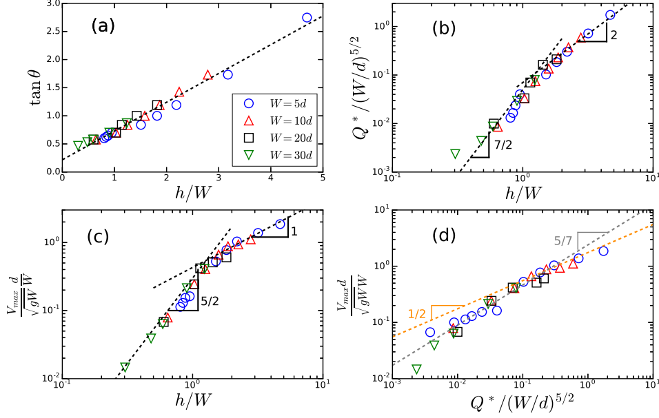
FIGURE 9. (a) The tangent of the angle of the flow depends linearly on the ratio h/W , where W is the gap between the sidewalls and h the depth of the flow determined by fitting the velocity profile (see text). (b) The dimensionless flow rate per unit width Q^* scales with (W/d)^{5/2} at any angle. Its dependence with h/W is more complex: it is compatible with a (h/W)^{7/2} scaling for angles below \theta_c \approx 40^\circ (regime I) and a (h/W)^2 scaling above (regime II). (c) Similarly, the maximal value of the velocity V_{max} scales with (W/d)^{3/2} at any angle and with (h/W)^{5/2} ( \theta < \theta_c , regime I) and h/W ( \theta > \theta_c , regime II). (d) The difference of scaling for the two regimes can also be confirmed by plotting V_{max}d/(W\sqrt{gW}) versus Q^*/(W/d)^{5/2} : the former quantity scales with the latter to the power 5/7 and 1/2 respectively for \theta < \theta_c and \theta > \theta_c .
