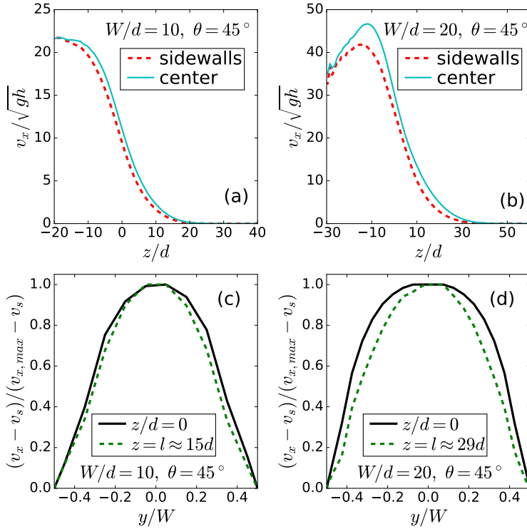
FIGURE 17. Effect of sidewalls on the velocity profiles for a flow angle equal to 45^\circ i.e. greater than \theta_c , the angle corresponding to the transition between regime I and regime II. For small gap width ((a) W/d = 10 ) the difference between the vertical velocity profiles at sidewalls and in the centre of the simulation cell is small and increases with increasing W ((b) W/d = 20 ). The influence of the sidewalls on the transverse profile of the reduced velocity at a given depth z (i.e. (v_x - v_s)/(v_{x,max} - v_s) where v_{x,max} and v_s are respectively the maximum velocity and the sliding velocity at the aforementioned depth) is weak but increases from the flow region to the creeping one. This variation with depth also increases with increasing W (c) and (d).
