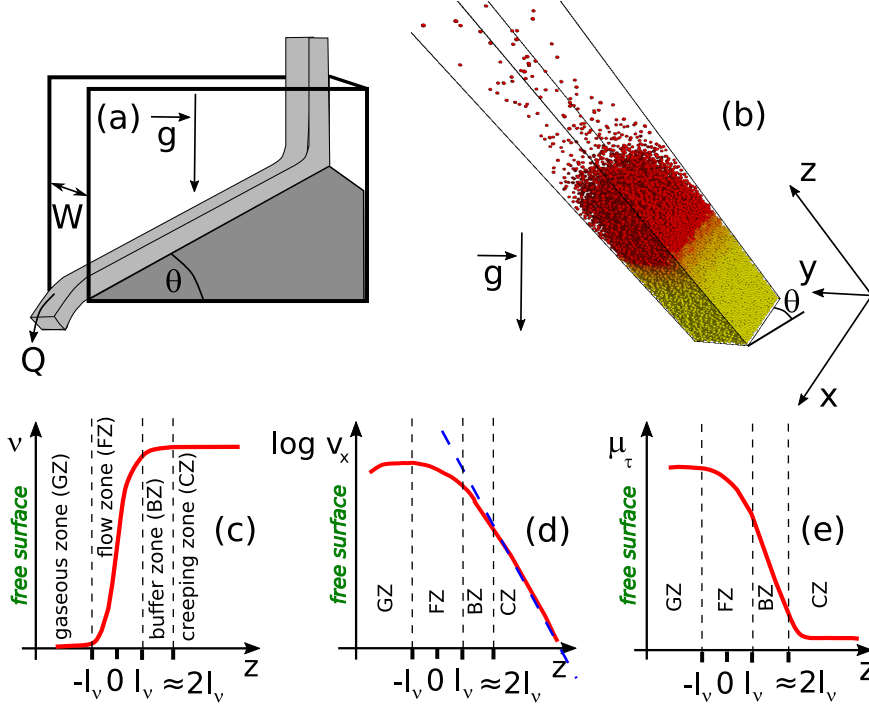
FIGURE 1. Sketch of the granular chute flow set-up: a surface flow occurs over a pile and is confined between two sidewalls separated by a gap W (a). The angle of the flow, \theta , increases with the flow rate Q . Typical three-dimensional snapshot for chute flow: W/d = 20 , N = 24,000 (b). Flow is directed down the incline along the x -axis and its angle is \theta = 45^\circ . The two sidewalls are parallel to the (xz) plane. The axes x , y and z are also reported and the origin is arbitrary. Sketches of the vertical profiles of the volume fraction \nu (c), logarithm of the streamwise velocity v_x (d) and sidewall friction \mu_\tau (e) obtained in Richard et al. (2008). The top and the bottom of the system correspond to z \rightarrow -\infty and z \rightarrow +\infty , respectively, and z = 0 is defined as the depth for which the volume fraction is equal to the half of its maximal value. The variation of the volume fraction is characterized by a length l_\nu which allows us to define four zones from top to bottom: (i) a dilute gaseous zone (GZ) located between -\infty and -l_\nu where particles have ballistic trajectories and experience rare collisions, (ii) a flowing zone (FZ) between -l_\nu and l_\nu where \nu rapidly increases with depth, (iii) a buffer zone (BZ) between l_\nu and approximately 2l_\nu and finally (iv), below the buffer layer, a creeping zone (CZ) where \nu = \nu_0 \simeq 0.6 .
