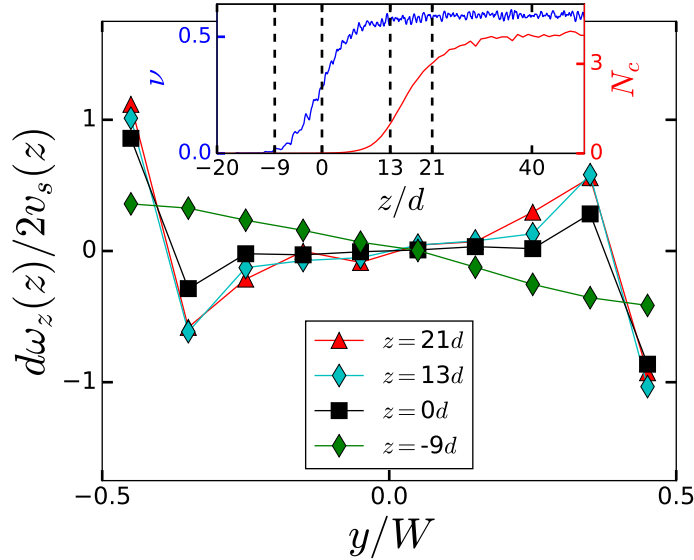
FIGURE 19. Profiles of vertical rotation velocity rescaled by 2v_s/d versus y for an angle \theta = 40^\circ and for several vertical positions. The gap between the sidewalls is W/d = 10 . For the sake of clarity, the inset reports the aforementioned vertical positions (dashed lines) on the vertical profiles of the number of contacts, N_c and of the volume fraction, \nu .
