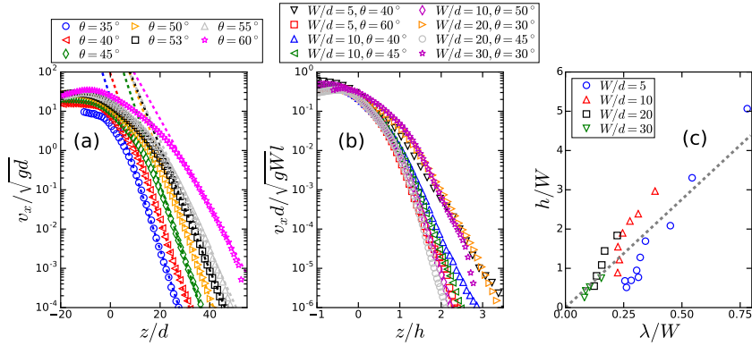
FIGURE 11. In the creeping zone, the velocity decays exponentially with the depth. This is illustrated in panel (a) for W/d = 10 . (b) Rescaling the velocity by \sqrt{gW}l/d and the depth by h leads to a collapse of the velocity profiles in the creeping region for \theta > \theta_c (b). The characteristic length of this decay, \lambda , is found to be correlated to the length h (c).
