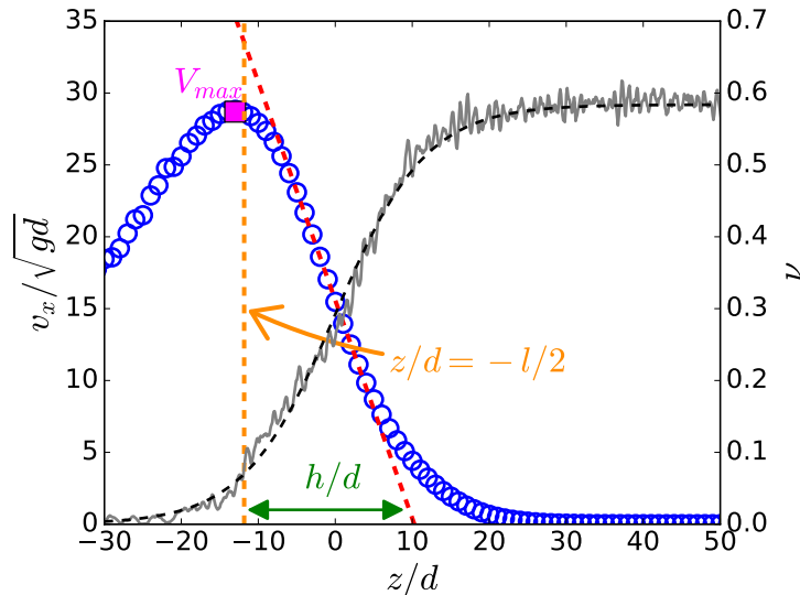
FIGURE 7. Velocity (blue open circles) and volume fraction profiles (grey line) and its fit by equation 4.1 (black dashed line) for W/d = 10 and \theta = 53^\circ . The height of the flow h is the distance between z = -l/2 (orange dashed vertical line, position corresponding approximately to V_{max} ) and the depth at which the tangent to the linear part of the velocity profile (dashed red line) intersects the z axis.
