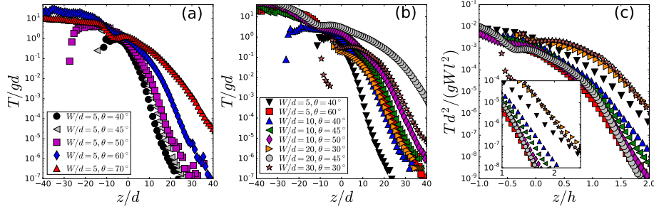
FIGURE 14. (a) For a given channel width (here W = 5d ) the vertical profiles of fluctuations of the particle velocity increase with \theta the angle of the flow. The vertical profiles plotted for various widths and angles can be rescaled using l as a length scale and h as a depth scale similarly to what is observed for the velocities (c). A zoom corresponding to low granular temperatures is reported in the inset of panel (c).
