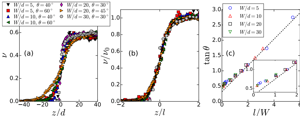
FIGURE 5. The vertical profiles of the volume fraction for various inclination angles \theta and widths W (a) collapse onto a master curve \nu(z) = \frac{\nu_0}{2} [1 + \tanh(2z/l)] –dashed line in panel (b). The characteristic length l scales with W and increases with the angle of inclination \theta (c). The dashed line represents the best linear fit for all the data. At low angle a slight deviation from the linear relation is found (inset of panel (c)). The angle for which this deviation is visible is close to \theta_c = 40^\circ and l/W \approx 1 . For this reason, the linear fit reported is done for angles above \theta = 40^\circ .
