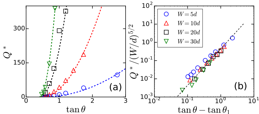
FIGURE 4. (a) For any gap between sidewalls W , the flow rate per unit width, Q^* , is found to increase with the angle of the free surface \theta . For a given \theta , increasing W leads to an increase of Q^* . (b) The flow rate per unit width can be rescaled by (W/d)^{5/2} . The evolution of the rescaled flow rate versus \tan \theta can be fitted by a quadratic law.
