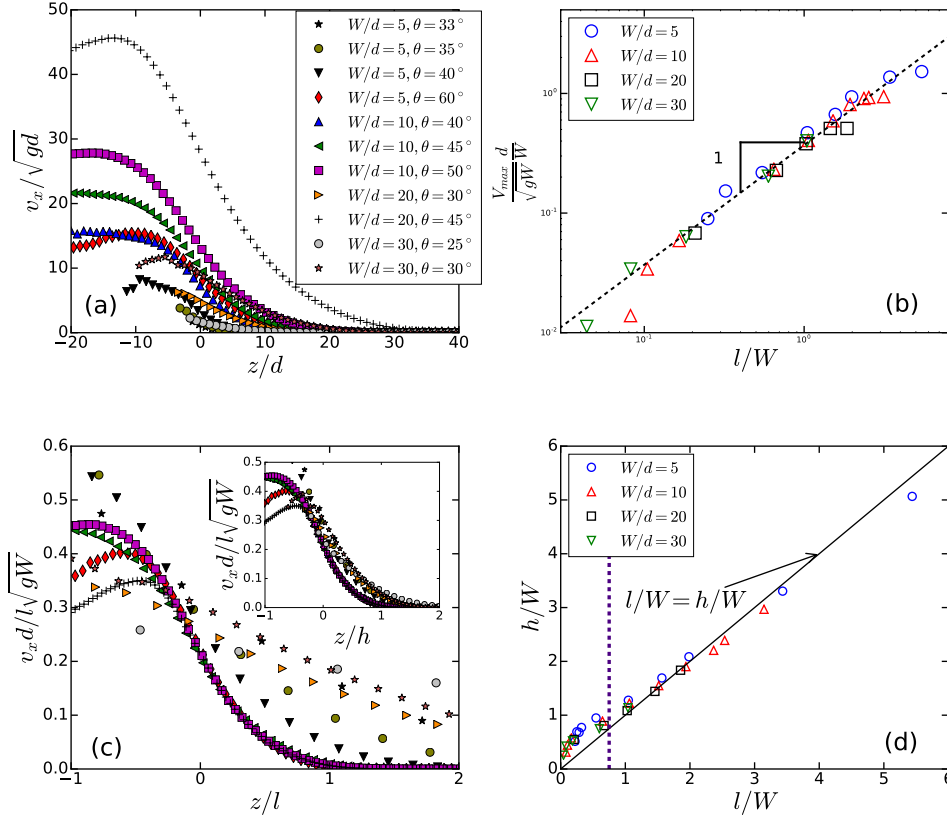
FIGURE 8. (a) Vertical profiles of the particle velocity in the main flow direction for various inclination angles \theta and widths W . (b) The maximal velocity (estimated by v_x(z = l/2) ) scales with the characteristic velocity \sqrt{gW}(l/d) . (c) Flows in regime II collapse onto a single curve when rescaling the velocity by \sqrt{gW}l/d and the depth by l or by h (inset of panel(c)). (d) In regime II, the characteristic length l determined by fitting the volume fraction profiles is close to h , the length determined through the velocity profile. In regime I, below \theta_c \approx 40^\circ important relative differences are observed (c).
