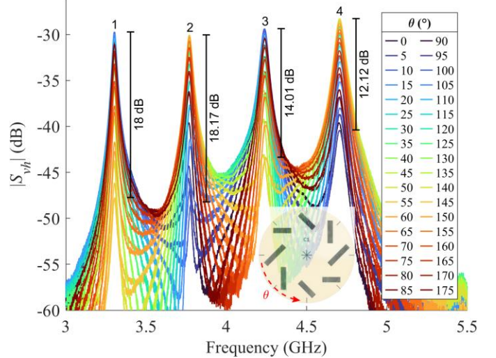
Fig. 16. Measured cross-polarization signals S_{vh} of C1 chipless RFID tag while varying the angle of rotation \theta from 0^\circ to 180^\circ . Inset: corresponding photograph of the chipless RFID tag.
