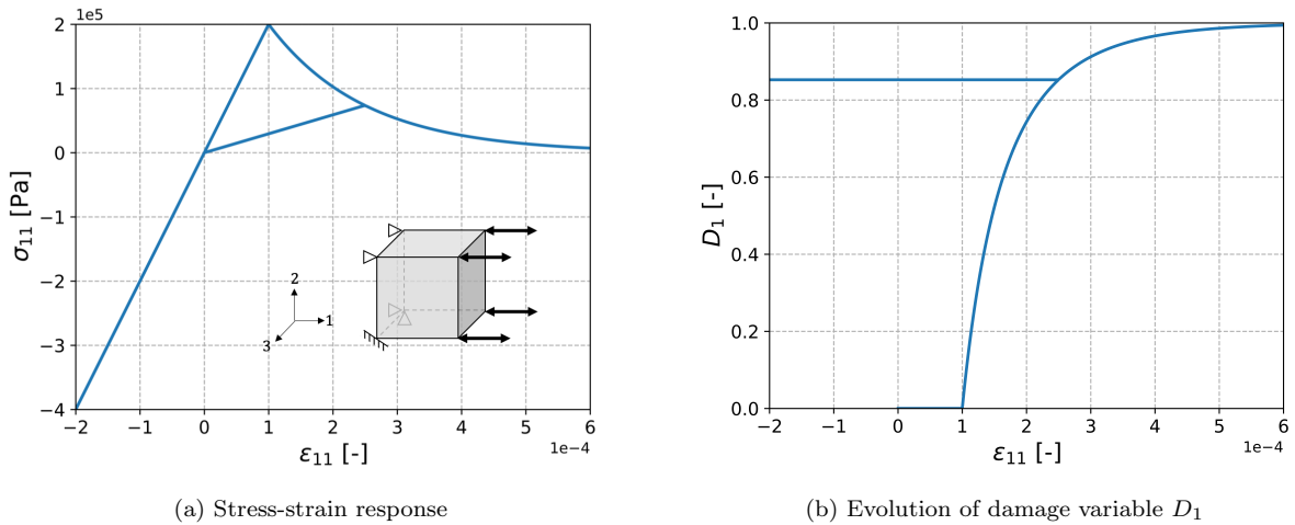
Figure 3: Unidirectional tensile/compressive test along direction 1
