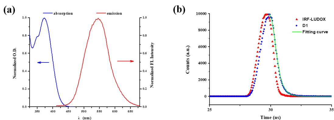
Figure 3. (a) Singlet state energy determination of D1; (b) Fluorescence decay curve of D1.
