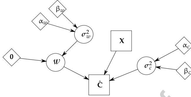
Figure 13: Hierarchical Bayesian model for the regression. Diamonds for hyper-parameters, rounds for parameters, squares for measurements. \hat{C} is the predicted variable sample, while X stands for the predictor variables sample. W is the weight matrix to infer, whose prior mean is 0 and variance \sigma_w^2 \in \mathbb{R}^{N_c \times N_{rb}} . The hyper-parameters of \sigma_w^2 are chosen by the user and noted \alpha_w and \beta_w . \sigma_c^2 \in \mathbb{R}^{N_c \times N_{bins}} contains the variances of the error \mathcal{E} , which are supposed to follow Inverse Gamma distributions of hyper-parameters \alpha_c and \beta_c .
