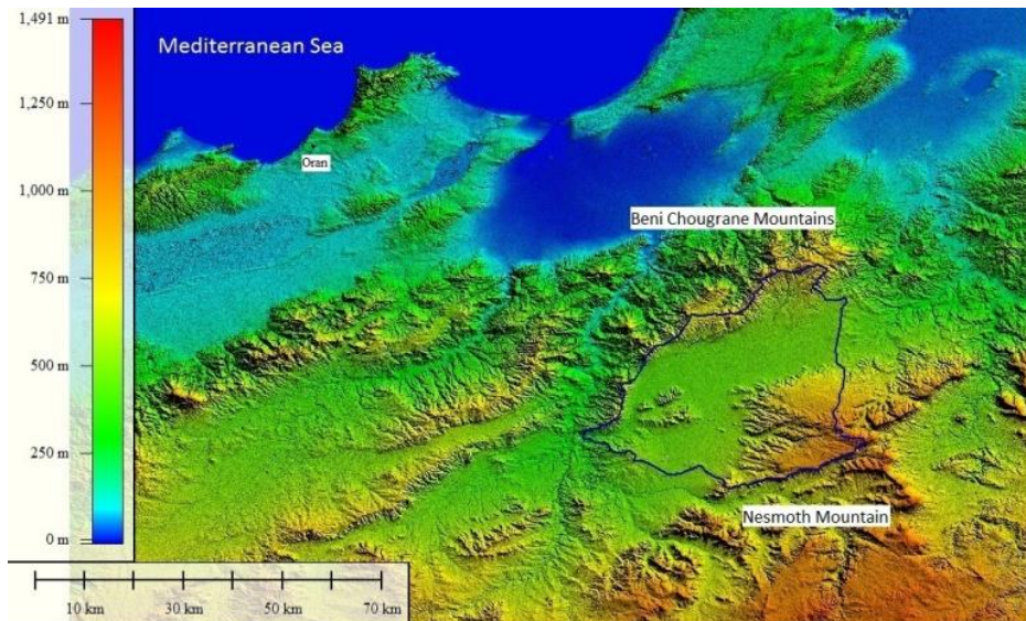
Figure 2. Digital Elevation Model of Oued Fekan.
