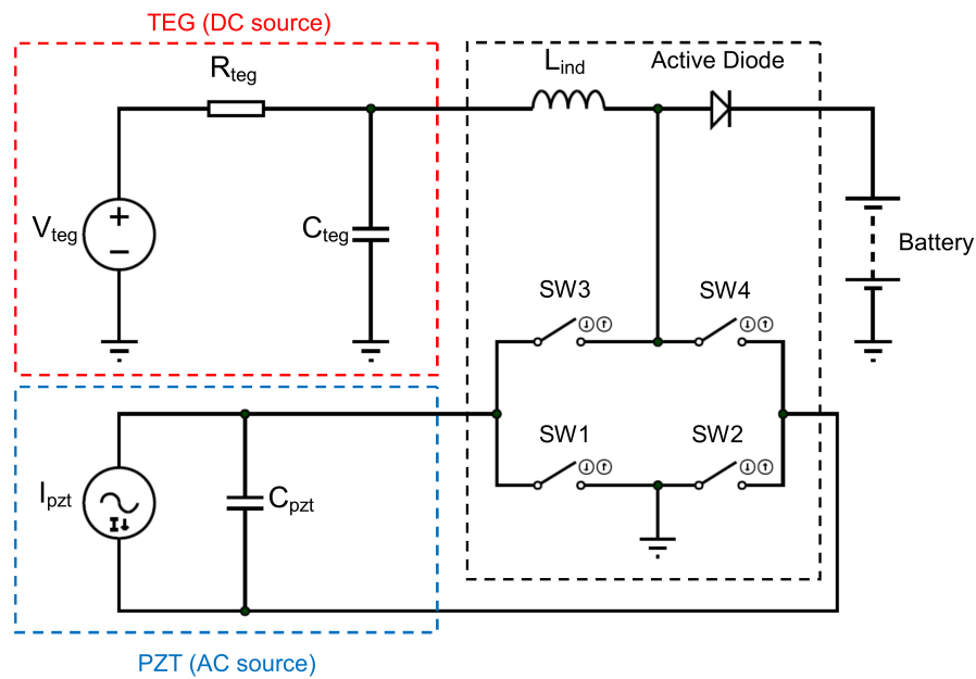
Fig. 10 The Yoon et al. harvester circuit [107]
