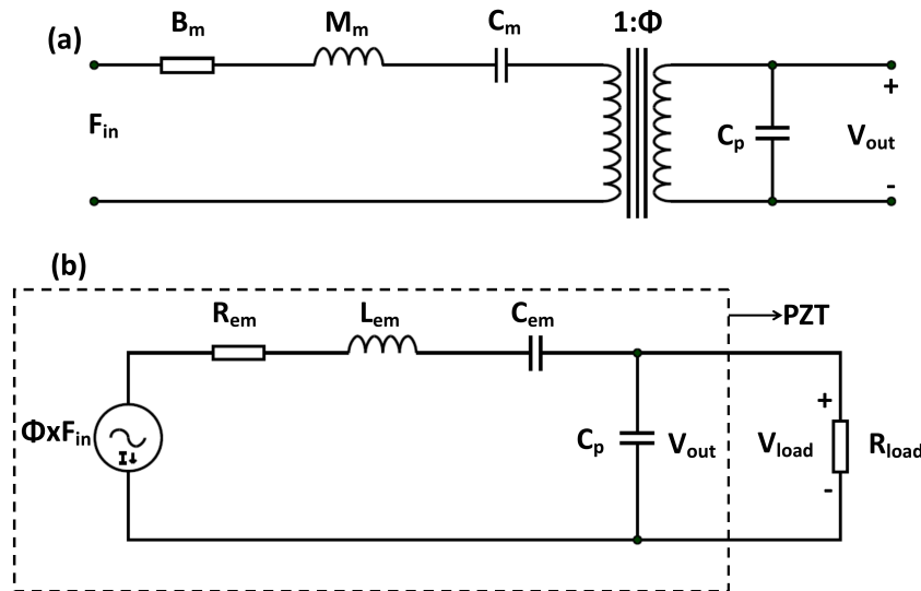
Fig. 4 Mechanical model (a) and equivalent electrical model (b) of a piezoelectric material [46], [48], [49]
