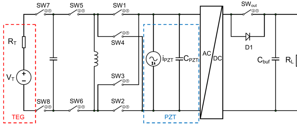
Fig. 11 The Li and al. harvester circuit [108]
