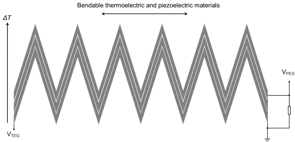
Fig. 13 Voltage measurement of Montgomery et al.'s harvester [112]
