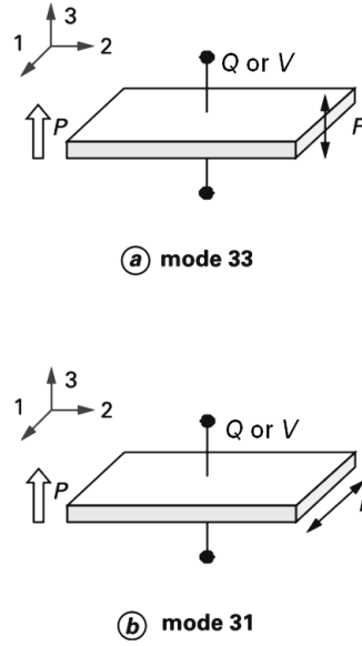
Fig. 2 Piezoelectric effect and deformation mode: (a) mode 33 , (b) mode 31
