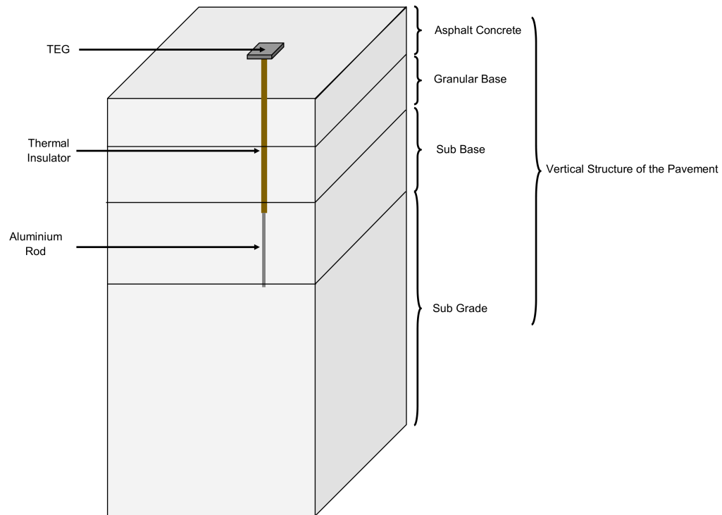
Fig. 9 Components of the Energy Harvest System and Vertical Structure of the Pavement [98]
