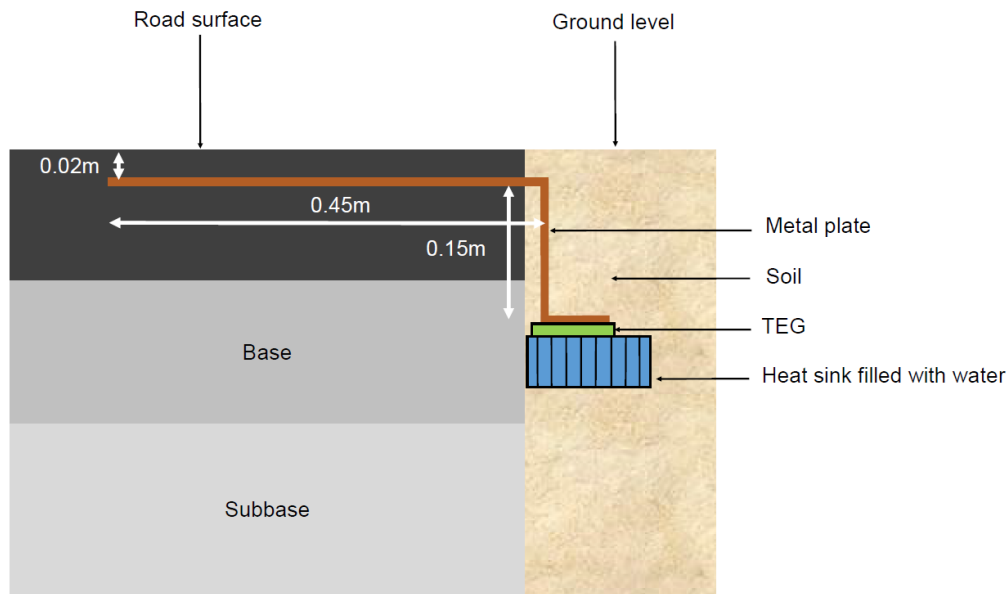
Fig. 8 Thermoelectric harvester prototype [95]
