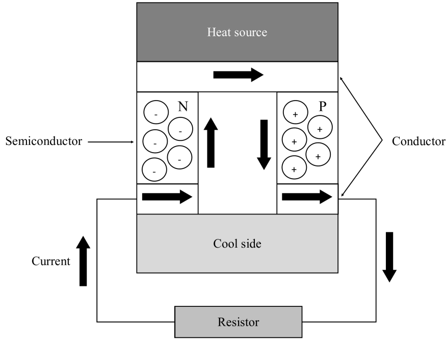
Fig. 3 Thermoelectric effect [33]
