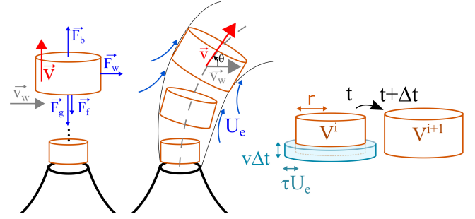
Figure 3: Left: Forces applied to a plume slice. Middle: Effect of wind on the path and orientation of slices. Right: Increase of slice volume at each time step, considering the entrained air represented by the blue ring.
