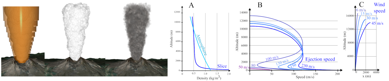
Figure 4: Left: Real-time previsualization of the column dynamics showing respectively the slices; the first and second scale spheres; rotating billboard. Right: Validation of the evolution of the simulation parameters. A: Evolution of the density of the column with respect to the altitude, compared to the density of the standard atmosphere (for a given ejection speed and no wind). B: Evolution of the altitude and vertical speed of a slice for different ejection speeds. C: Trajectory of a slice displayed in a 2D graph when a constant horizontal wind is applied. Stronger wind velocity leads to a lower maximal altitude.
