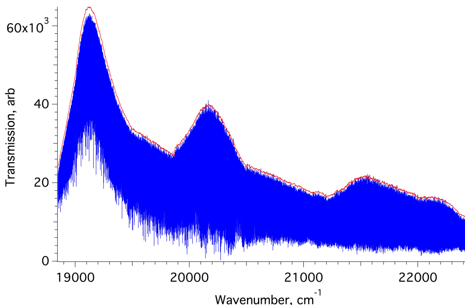
Figure 2. Overview of the composite transmission spectrum recorded with the visible beamsplitter, the contour being imposed by selections of optical filters. The continuous trace above (red) represents the baseline used to generate a transmittance spectrum.
