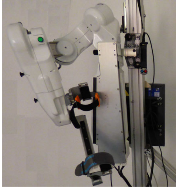
Fig. 1. Picture of the 4D ABLE exoskeleton used in this study.
