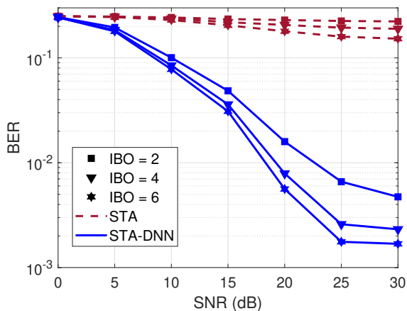
(b) STA and STA-DNN estimators.
