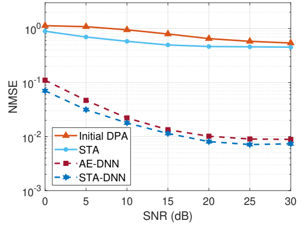
(b) With HPA nonlinearities and IBO = 4 dB.
