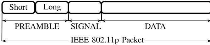
Fig. 1: IEEE 802.11p packet structure [1].
