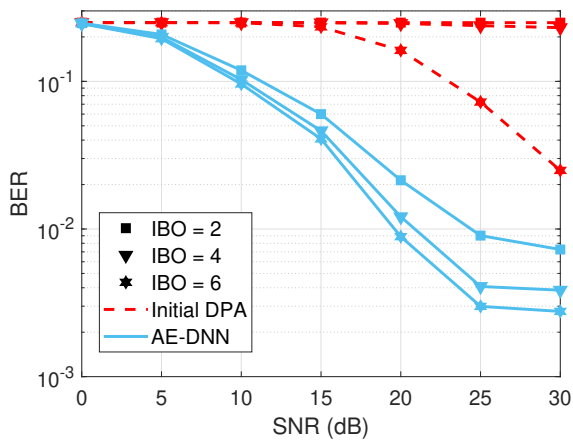
(a) Initial DPA and AE-DNN estimators
