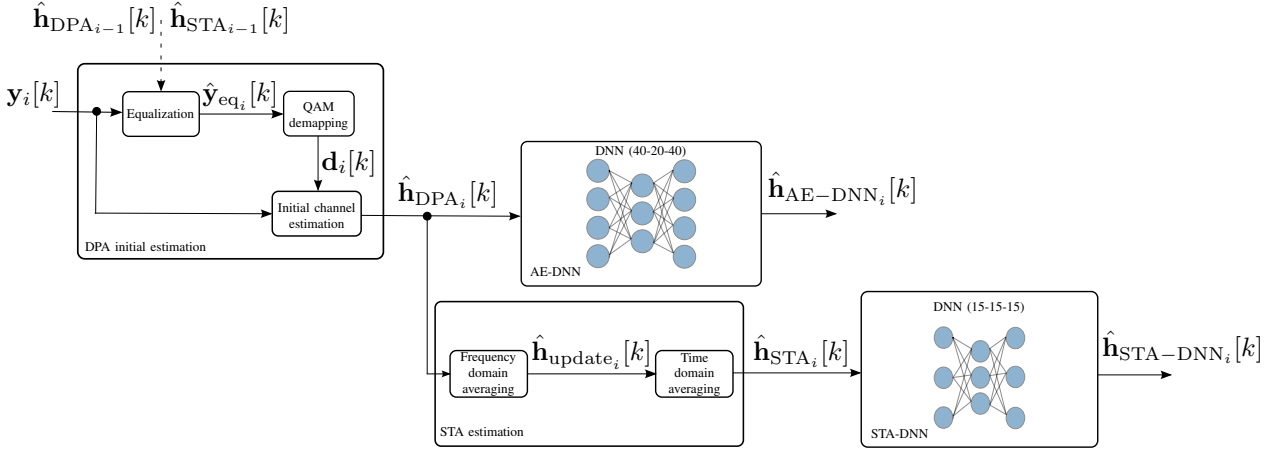
Fig. 2: Block diagram of the DNN-based estimators: AE-DNN and STA-DNN.
