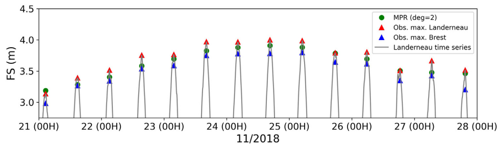
Figure 7 Time series of free-surface elevation observed in Landerneau with observations in Brest and predictions in Landerneau (from MPR with \text{deg}=2 ) of maxima reached during high tides during spring tidal conditions. These comparisons were shown over the initial validation dataset.
