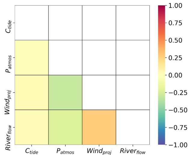
Figure 6 Matrix of Spearmann correlation coefficients between input features of machine learning algorithms. Results are naturally shown for the lower part of this symmetrical matrix.
