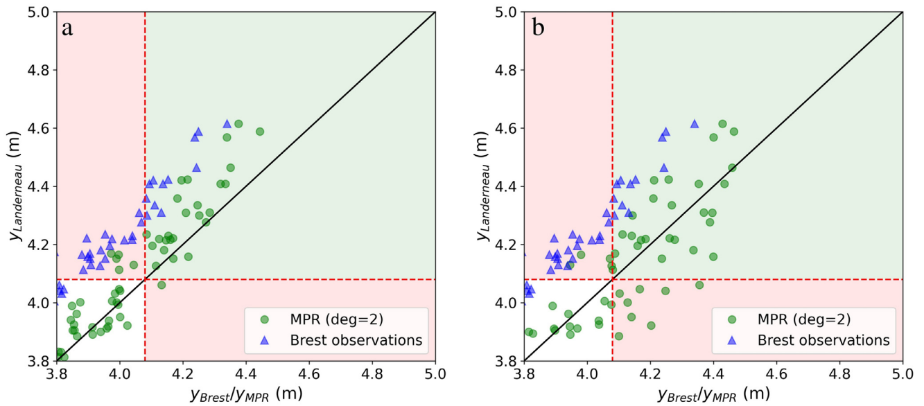
Figure 12 Correlation between observed and predicted maxima during high tides in the city of Landerneau from MPR with \text{deg}=2 for (a) C_{\text{tide}} and P_{\text{atmos}} and (b) C_{\text{tide}} as input variables. Correlation between maxima observed in Landerneau and in Brest harbour are shown with blue triangles. These different values were shown for the new tested dataset corresponding to the final 30% of observations over the period 02-03-2017/25-06-2020.
