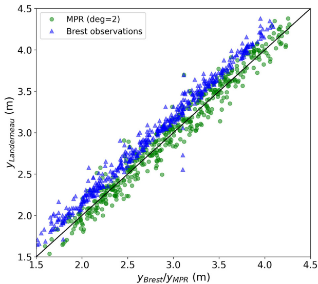
Figure 8 Correlation, over the initial validation dataset, between maxima observed and predicted (from MPR with \text{deg}=2 ) during high tides in the city of Landerneau (green circles). Correlation between maxima observed in the city of Landerneau and observed in Brest harbour (blue triangles).
