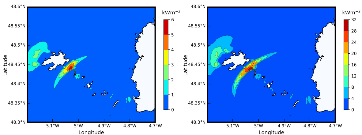
Figure 5. Cartography of (left) averaged and (right) maximum kinetic power density during a spring-neap tidal cycle (T = 14.765 days) resulting from M 2 , S 2 and M 4 harmonic components (adapted from [3]).
