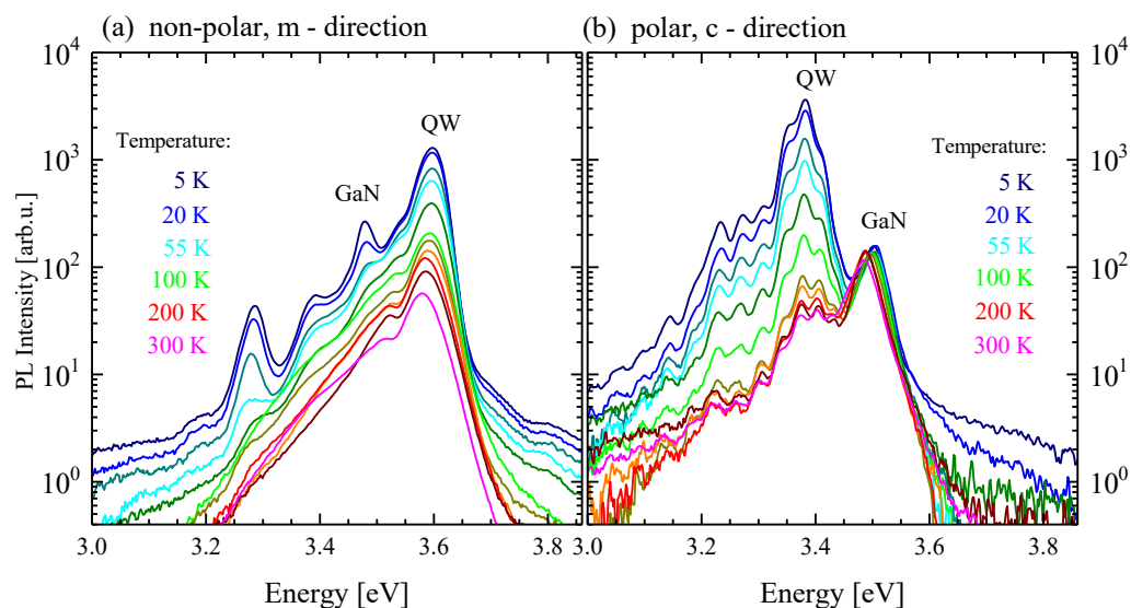
Figure 5. The temperature dependence of PL spectra of (a) non-polar and (b) polar GaN/Al 0.26 Ga 0.74 N (3 nm/22.5 nm) MQW structures. The oscillations visible in Panel (b) are due to reflection at the GaN/Si interface and the resulting Fabry-Pérot interferences.
