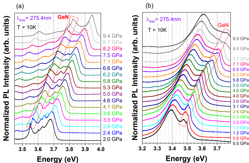
Figure 10. Pressure dependence of the low-temperature PL spectra of a non-polar (a) and polar (b) GaN/AlGaIn MQWs. The emission from the GaN cap (marked by red tetragons) is visible in the whole range of pressures.
