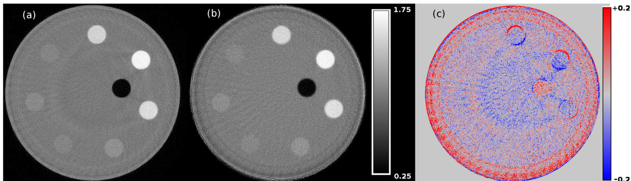
FIGURE 3 Reconstructed RSP images with 0.2 mm × 0.2 mm pixel size from (a) the phase-II and (b) the pVDA scanner. The average of 20 central slices was taken to reduce noise and the images are shown with an RSP level of 1.0 and window of 1.5. In (c), the difference (b)–(a) is shown with an RSP level of 0 and window of 0.4
