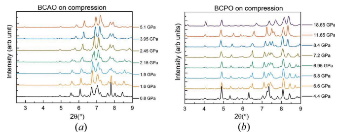
Figure 2 (a) Synchrotron X-ray diffraction patterns of B CAO from 0.8 GPa up to 5.1 GPa at room temperature on compression. (b) Synchrotron X-ray diffraction patterns of BCPO from 4.4 GPa up to 18.65 GPa at room temperature on compression.
