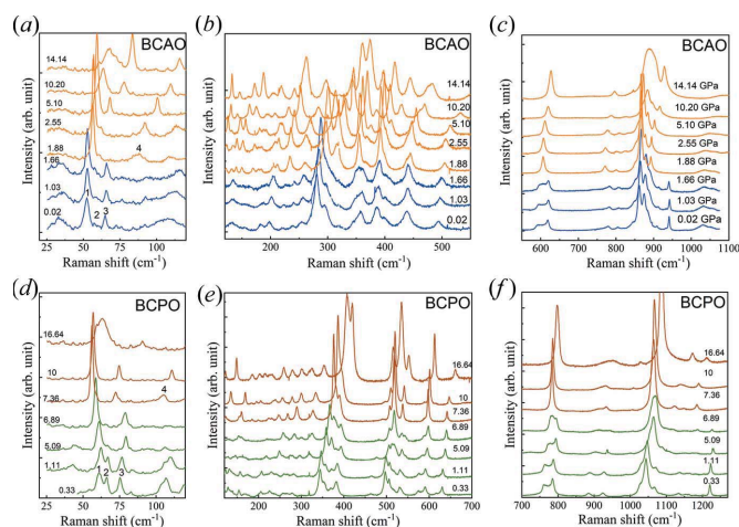
Figure 8 Evolution of the Raman spectra measured in BCAO and BCPO at selected pressures are shown in three different regions with different scaling. Raman spectra at different pressures recorded on compression. Representative Raman spectra of barium cobalt arsenate on compression up to 14.14 GPa: (a) between 25 and 120 \text{cm}^{-1} , (b) between 120 and 580 \text{cm}^{-1} and (c) high-frequency region between 580 and 1080 \text{cm}^{-1} . Representative Raman spectra of barium cobalt phosphate on compression up to 16.64 GPa: (a) between 25 and 160 \text{cm}^{-1} , (b) between 120 and 700 \text{cm}^{-1} and (c) high-frequency region between 700 and 1280 \text{cm}^{-1} . The two-colour representation is used to distinguish between the low-pressure and the high-pressure phases.
