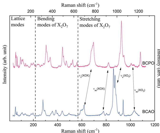
Figure 7 Raman spectra of BCPO and BCAO recorded at atmospheric pressure and room temperature. The three frequency divisions, separated by dashed lines, represent lattice modes of \text{BaCoX}_2\text{O}_7 ( X = \text{As, P} ), bending modes of \text{X}_2\text{O}_7 ( X = \text{As, P} ) double tetrahedra unit and stretching modes of \text{X}_2\text{O}_7 . BCPO scale belongs to the upper x axis and BCAO scale belongs to the lower x axis.
