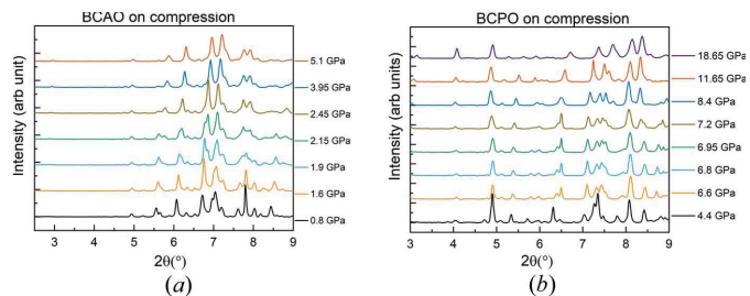
Figure 2 (a) Synchrotron X-ray diffraction patterns of BCAO from 0.8 GPa up to 5.1 GPa at room temperature on compression. (b) Synchrotron X-ray diffraction patterns of BCPO from 4.4 GPa up to 18.65 GPa at room temperature on compression.
