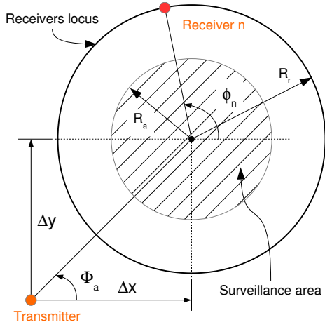
Fig. 1. Multistatic configuration.
