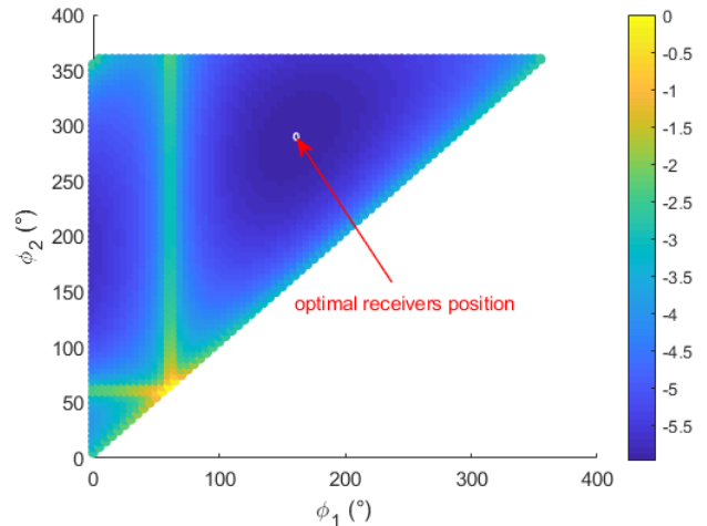
Fig. 2. Normalized trace of CRLB (dB) for one given target configuration.
