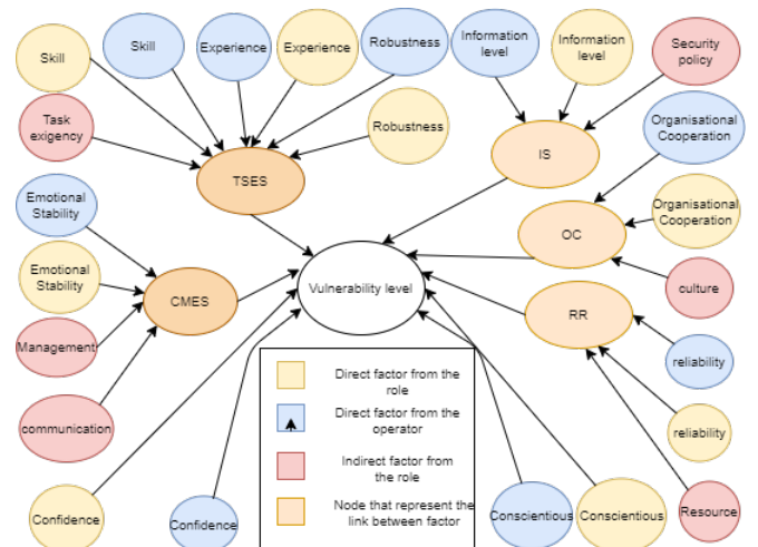
Fig. 1. Bayesian network for estimating operator's vulnerability level.
