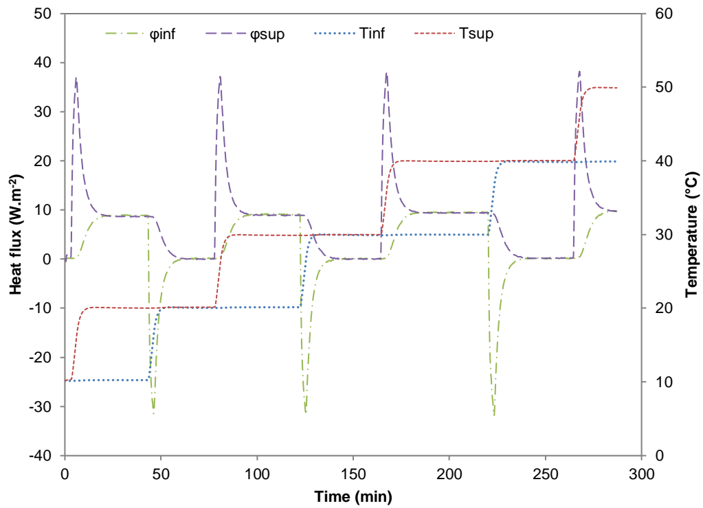
Figure 7- Measured temperatures and heat fluxes at the upper and bottom sample faces
