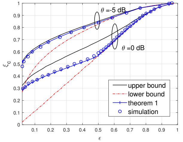
Figure 3. The approximation and bounds of the \epsilon -stable region.
