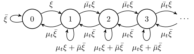
Figure 1. DTMC model.
