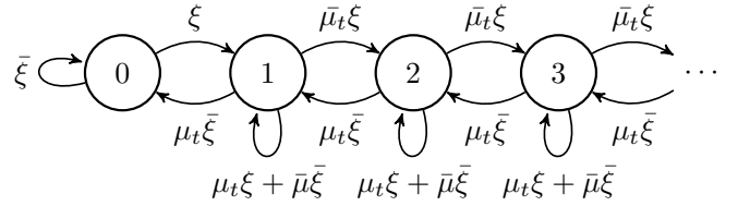
Figure 1. DTMC model.
