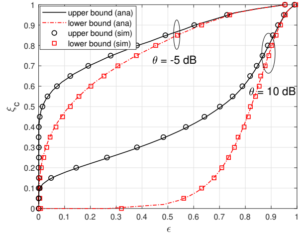
Figure 2. Upper and lower bounds of the \epsilon -stable region.
