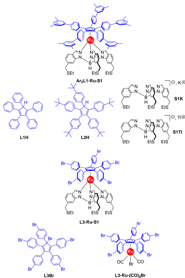
Scheme 1. Structures of the two molecular rotors Ar 3 L1-Ru-S1 and L3-Ru-S1 , along with their related ligands or fragments.
