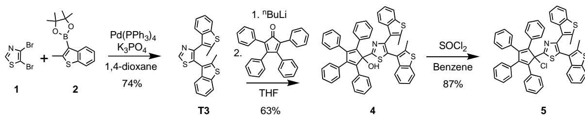
Scheme 1. Synthesis of the cyclopentadiene rotor functionalized with a terarylene fragment (5).
