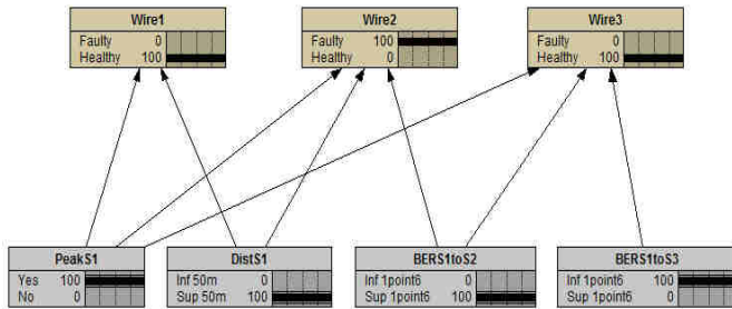
Fig. 8. The Bayesian Network Structure
