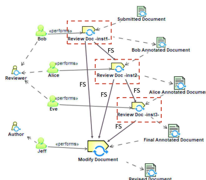
Fig.2: Sequential strategy of the collaborative task Review Document
