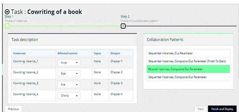
Fig.4: Screenshot of a task deployment: Cowriting of a book - left side: list of task instances; right side: the choice of a collaboration pattern.
