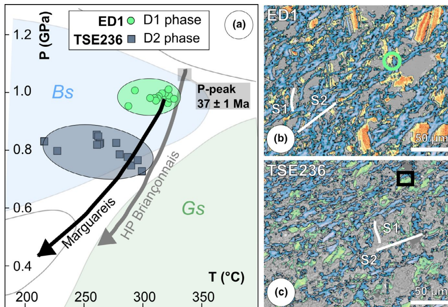
FIGURE 5 (a) P - T path of the Marguareis Unit (black arrow in the P - T space) obtained in this study. The paths related to the HP Briançonnais (grey arrow) are also plotted (data from Michard et al., 2004). The microdomains, in which the Chl-Phg couples used to constrain the P - T conditions of D1-D2 phases were sampled, are evidenced (b) in the sample ED1 with the green circle and (c) in the sample TSE236 with black rectangle. In (b) and (c), chlorite shadows are referred to the Fe-content (green-yellow-red colours) and phengite shadows represent the K-intensity (blue to white colours); other mineral phases (quartz, calcite, titanite and feldspar) are in grey
