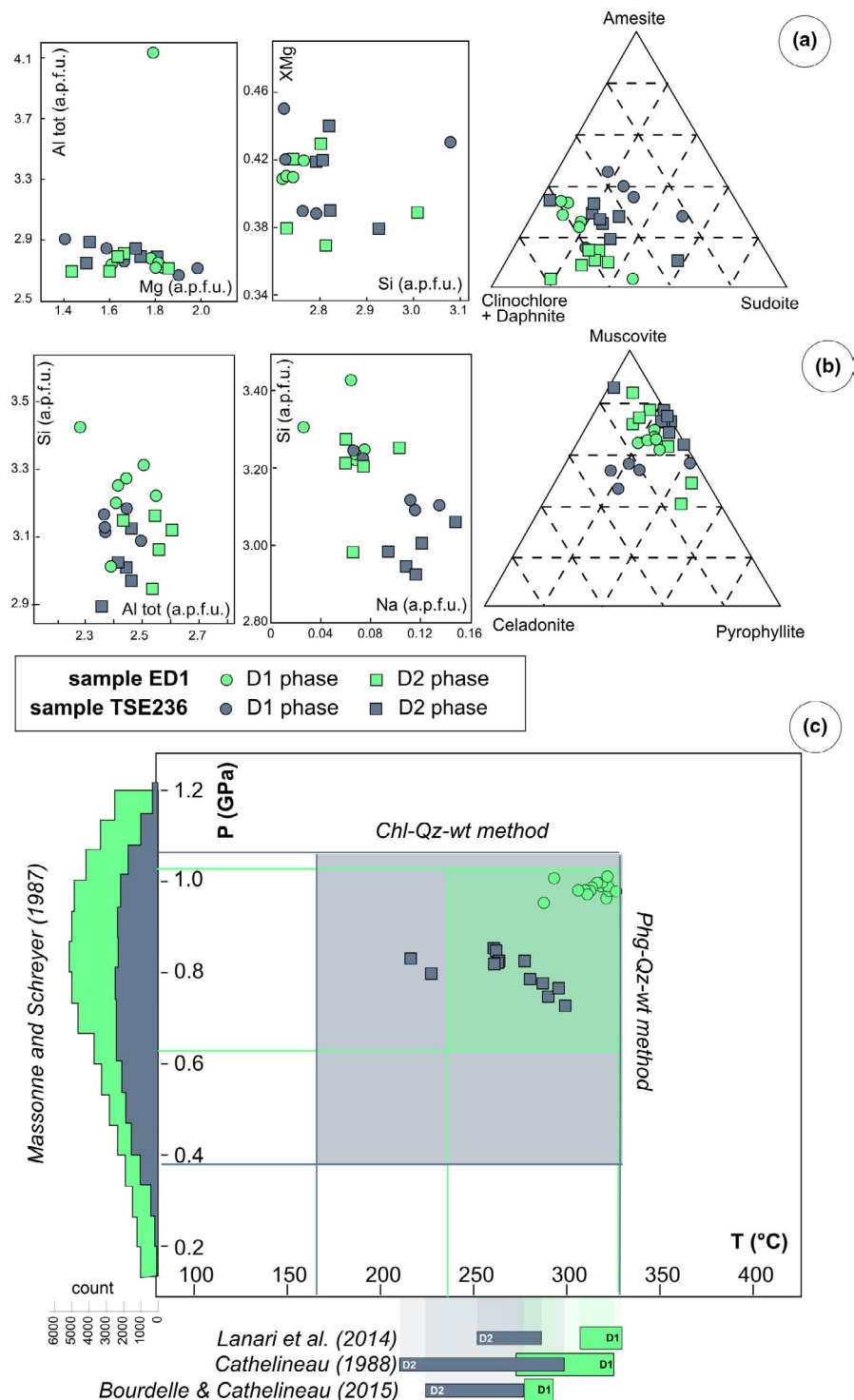
FIGURE 4 Geochemistry of (a) chlorite and (b) phengite sampled into ED1 and TSE236. Chlorite and phengite structural formula are calculated assuming 14 and 11 oxygen, respectively. (c) P/T diagram showing the results of the thermobaric methods applied to samples ED1 and TSE236. In the P/T space, the pale squares indicate the areas constrained by the Chl–Qz–wt method (Vidal et al., 2006) and the Phg–Qz–wt method (Dubacq et al., 2010); the position of data indicates the P–T equilibrium conditions of single Chl–Phg couples obtained with Chl–Phg–Qz–wt method (Vidal & Parra, 2000). Histograms along the Y-axis indicate the results of Massonne and Schreyer (1987) geobarometer. Along the X-axis, the used thermometers are reported with range values related to D1 and D2 phases
