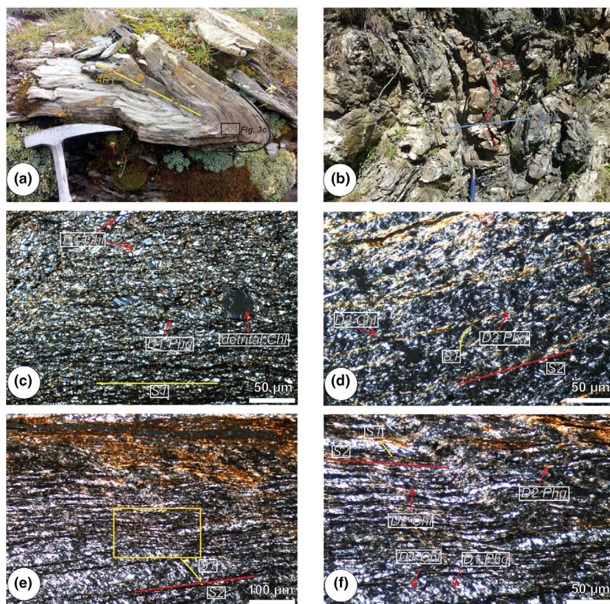
FIGURE 3 Meso- and micro-scale D1- and D2-related structural features of the Marguareis Unit. F1 and F2 folds (a, b) in the middle Eocene meta-pelites. (c–f) Microphotographs of the S1 and S2 foliations. The cross-cutting relationships are reported. AP1: F1-related axial plane; AP2: F2-related axial plane; AP4: F4-related axial plane
