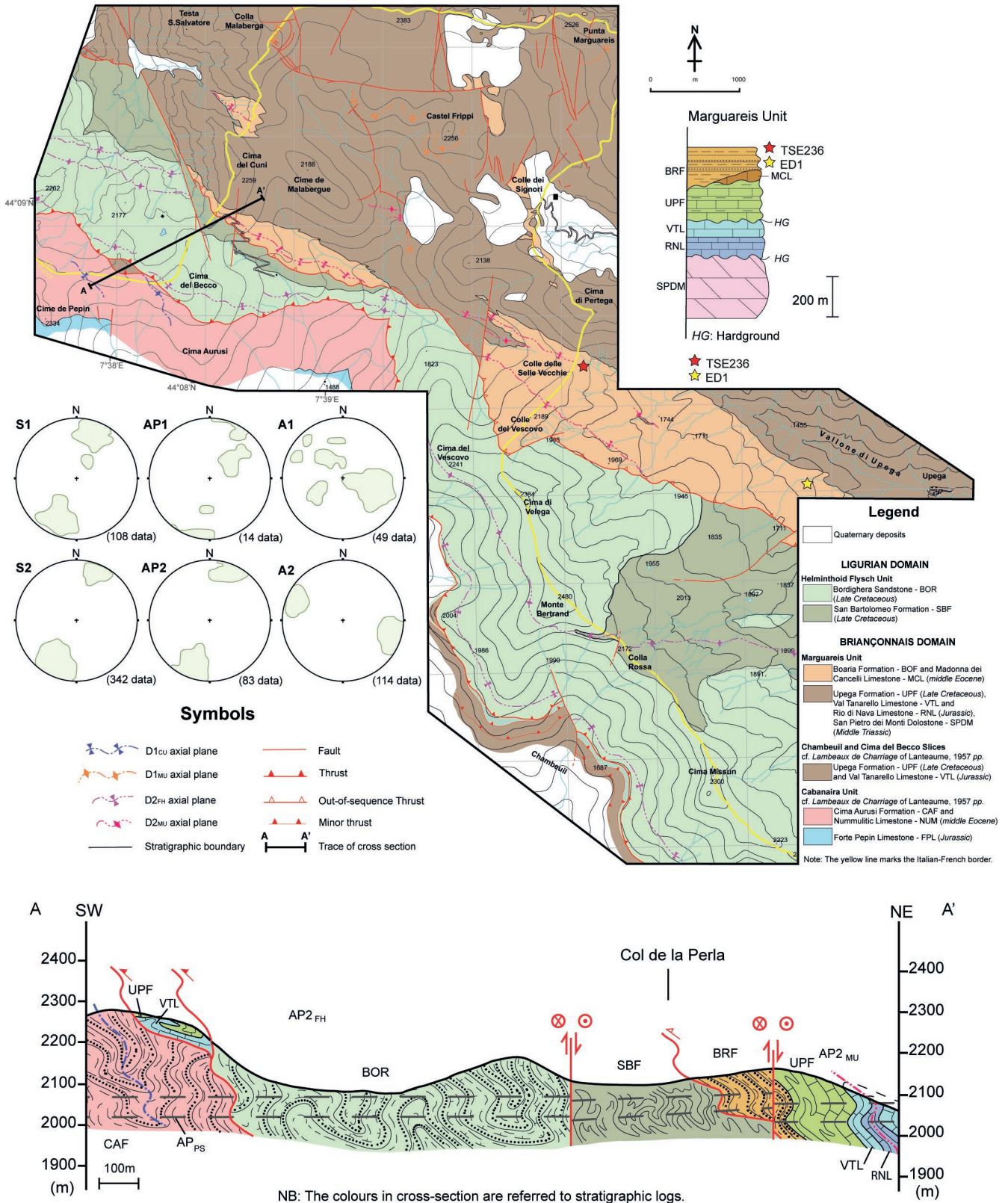
FIGURE 2 Structural sketch of the south-western sector of the Marguareis Massif with geological cross-section. Stereographic plots show the spatial relationships between planar and linear structural features recognized in the Marguareis Unit. The stratigraphic log (Middle Triassic–Middle Eocene age) of the Marguareis Unit is reported on the right corner (by Sanità et al., 2020). Red and yellow stars indicate the sample location
