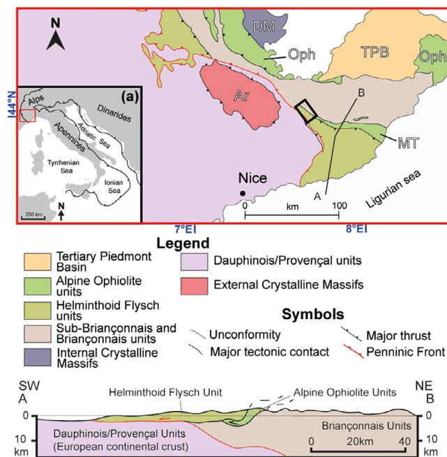
FIGURE 1 (a) Geographic location of the study area. (b) Simplified geological sketch of the South-Western Alps (modified and redraw by Molli et al., 2010) with regional-scale geological cross-section (redraw and modified from Bonini et al., 2010). Black box indicates the study area of Figure 2. In the cross-section, red line indicates the Penninic front. TPB, Tertiary Piedmont Basin; Oph, Alpine Ophiolitic Units; MT, Mglio-Testico Unit; DM, Dora Maira Massif; Ar, Argentera Massif
