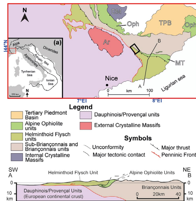
FIGURE 1 (a) Geographic location of the study area. (b) Simplified geological sketch of the South-Western Alps (modified and redraw by Molli et al., 2010) with regional-scale geological cross-section (redraw and modified from Bonini et al., 2010). Black box indicates the study area of Figure 2. In the cross-section, red line indicates the Penninic front. TPB, Tertiary Piedmont Basin; Oph, Alpine Ophiolitic Units; MT, Mglio-Testico Unit; DM, Dora Maira Massif; Ar, Argentera Massif
