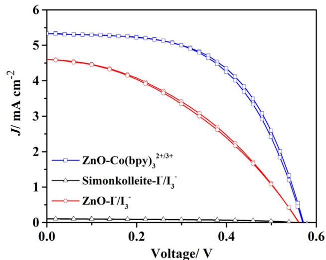
Figure 5. Current density vs voltage curves (forward and backward scan) for the best DSSCs elaborated with simonkolleite and ZnO films sensitized for 3 h in a MG-207 dye + CDCA solution at a scan rate of 50 \text{ mV s}^{-1} . Two electrolyte solutions are compared, based on the \text{Co}(\text{bpy})_3^{2+/3+} and the \text{I}^-/\text{I}_3^- redox couple, respectively.
