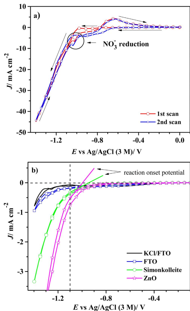
Figure 1. Cyclic voltammetry for electrolyte solutions purged with N_2 at pH 6 and at 70^\circ C , in the potential window from 0 to -1.4 V vs Ag/AgCl (3 M) and at a scan rate of 5 mV s^{-1} : (a) 0.1 M Zn(NO_3)_2 \cdot 6H_2O + 0.1 M KCl aqueous solution at FTO; (b) 0.2 M NaNO_3 + 0.1 M KCl aqueous solution at different electrodes.
