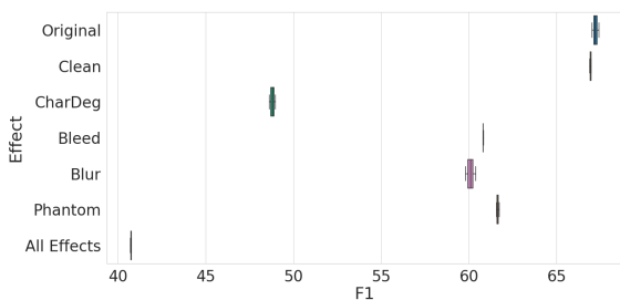
Fig. 18 The distribution of the CNN-based model F1 scores on the noisy test ACE 2005 for event classification .
