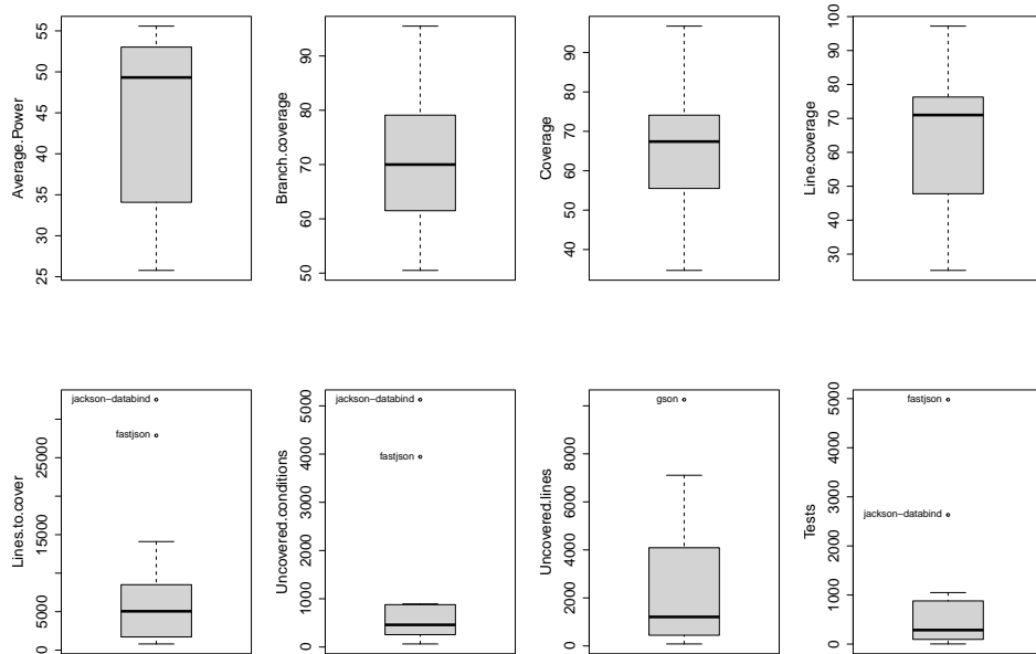
Figure 1. Distribution of values for each metric
