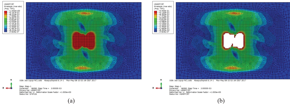
FIGURE 5. The matrix Hashin damage (a). Damaged elements removed (b)
