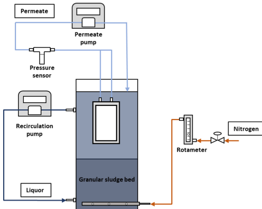
Fig. 1. Schematic representation of the experimental set-up used for the short- and long-term filtration tests.
