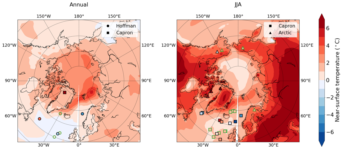
Figure 2. LIG-PI anomaly of the near-surface air temperature (°C) simulated by the IPSL-CM6A-LR model (colour shading) and reconstructed from proxy data synthesis (filled markers) as published by Otto-Bliesner et al. (2021). Symbols represent the source of surface air reconstruction: circles for the compilation by Hoffman et al. (2017), squares for the compilation by Capron et al. (2014, 2017) and triangles for the Arctic compilation. Sites showing good model–data agreement (i.e. considering a data uncertainty of \pm 1\sigma ) are indicated by a green outline.
