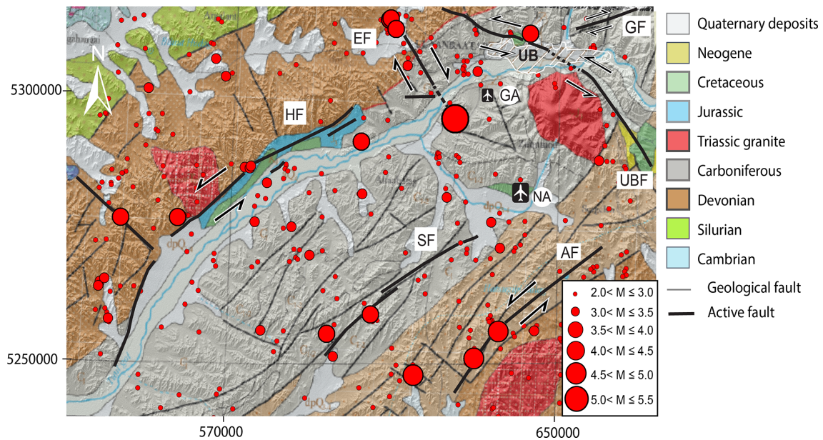
Figure 2. Geological and seismo-tectonic context of the Ulaanbaatar region. Red dots are earthquakes recorded between 1994 and 2011 (Institute of Astronomy and Geophysics, Mongolian Academy of Sciences, National Data Center). Black lines represent the active faults (HF: Hustai fault, EF: Emeelt fault, SF: Sharkhai fault, AF: Avdar fault, UBF: Ulaanbaatar fault, GF: Gunj fault). UB: Ulaanbaatar city, GA: Ghingis Khan old international airport, NA: new international airport. The background DEM is from SRTM1 data (see data and resources). Geological map is an extract from the geologic map of Mongolia (scale 1 : 1 M) (Tomurtogoo et al., 1998).
