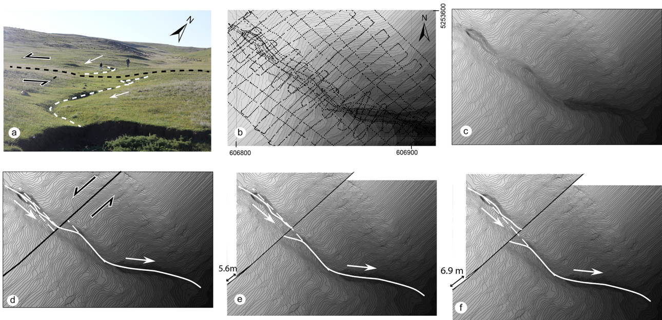
Figure 8. Offset reconstruction for drainage P2. (a) Field photograph of P2: the black dashed line indicates the fault trace. The north direction in the photograph is approximate. (b) Differential GPS measurements used to build the digital topographic map. (c) Digital topographic map based on GPS measurements. (d) Present-day situation: the offset is measured on images by projecting the average upstream and the downstream to the fault trace. We consider for the upstream a “wide zone” giving an uncertainty on its piercing position for the back-slip reconstruction. (e) Minimum back-slip reconstruction of 5.6 m. (f) Maximum back-slip reconstruction of 6.9 m. Hence, the left-lateral offset is estimated at 6.25 \pm 1.65 m. White arrows: water flow direction. For location, see Fig. 3.
