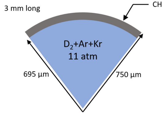
FIG. 1. Schematic design of the cylindrical targets, showing the plastic shell and the gas fuel. This cylinder is 3 mm long and the thickness of the CH shell is 55 \mu\text{m} .
