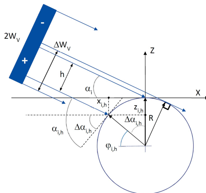
Figure 3 Detailed scheme of the incidence beam with a vertical size 2W_v as defined by slits before the sample as it impinges on the curved surface with the definition of angles used in formulas. The incident beam comes from the left. Narrow blue lines represent elementary rays. Here, h is the offset of the elementary ray from the beam center. This ray impinges with the circular surface of radius R at the point with coordinates (x_{i,h}, z_{i,h}) . The angle a_i is the effective grazing angle, while a_{i,h} and \Delta a_{i,h} are the actual grazing angle at the point (x_{i,h}, z_{i,h}) and the difference of this angle from a_i , respectively.
