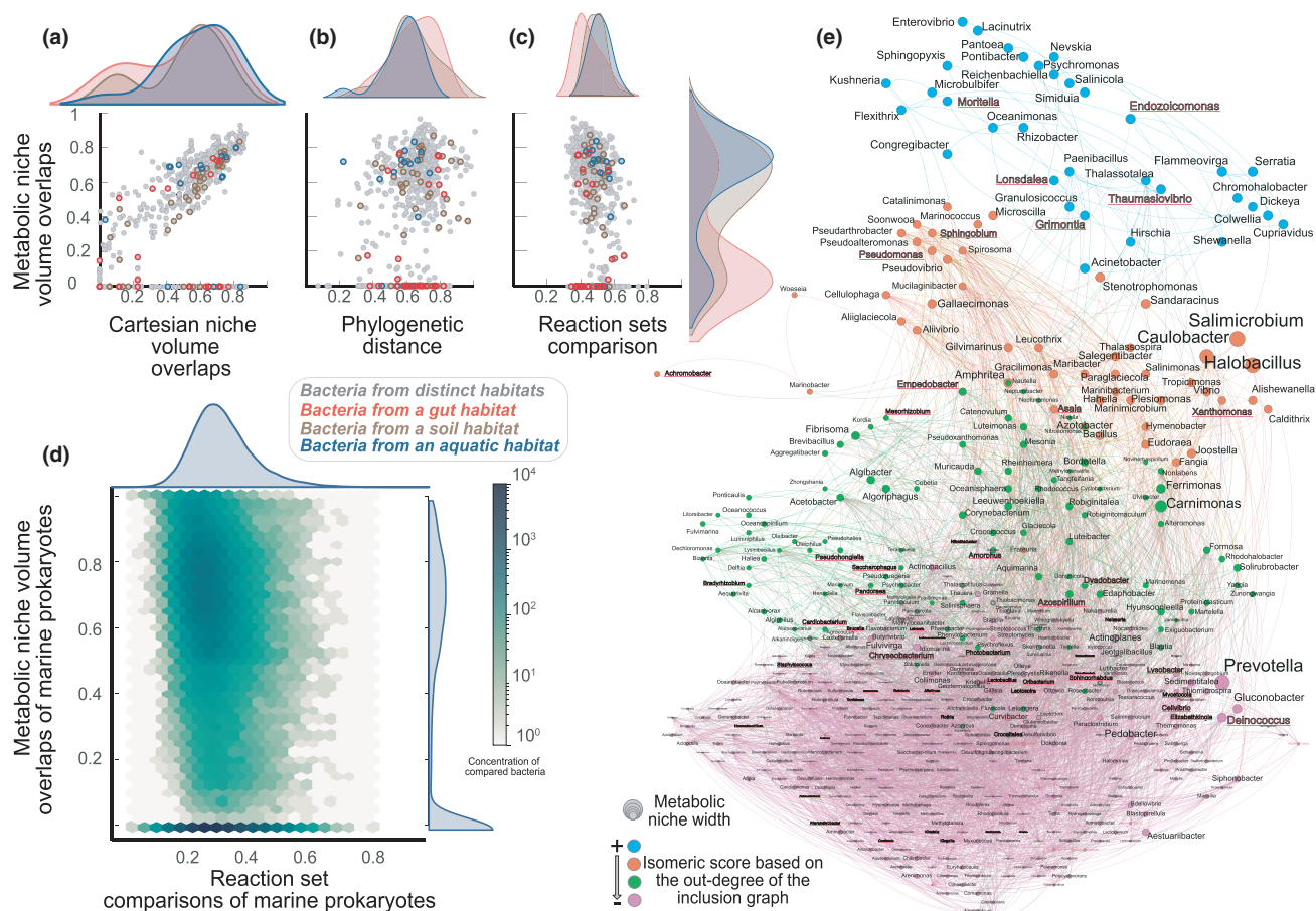
FIGURE 2 Comparison of the metabolic niche overlap with other pairwise distances and niche inclusion. (a) Comparison between metabolic niche overlaps and Cartesian niche overlaps estimated with a Jaccard distance. This comparison is performed for bacteria from different or common habitats. (b) Absence of a relationship between metabolic niche overlaps and pairwise phylogenetic distances based on 16S rRNA gene. (c) Absence of a relationship between metabolic niche overlaps and presence-absence of common reactions estimated via a Jaccard distance. (d) Absence of a relationship between metabolic niche overlaps and presence-absence of common reactions estimated for 502 marine bacteria metabolic models. Instead of a scatter plot, it shows concentrations for more than 10^5 pairwise comparisons. For bacteria that show metabolic niche overlaps almost null, we investigate potential niche inclusion. (e) Metabolic niche inclusion graph of marine bacteria. The node size is proportional to metabolic niche volume, and an edge indicates a metabolic niche's inclusion into another. The graph layout follows an isomeric distribution driven by the out-degree of the inclusion graph. Bacteria are divided into four categories based on the z-score from most embedded metabolic niche (i.e. turquoise) to the least (i.e. purple). Labels of bacteria known for being associated with a host are in red/bold and underlined
