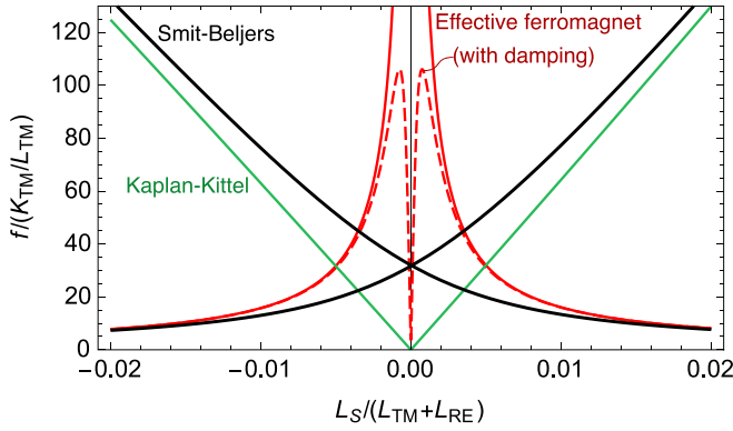
FIG. 5. Normalized absolute mode frequencies vs normalized angular momentum near angular compensation in a high-symmetry configuration calculated by different models: effective ferromagnet model with and without damping [12], the exchange coupling mode solution by Kaplan and Kittel [33], and the double-lattice Smit-Belgers model described before. The magnetization and anisotropy axis are parallel. The parameters (J, K_i, g_i) are those of Table I, except for \alpha_{\text{TM}} = 0.0015 . All other energy terms are neglected.
