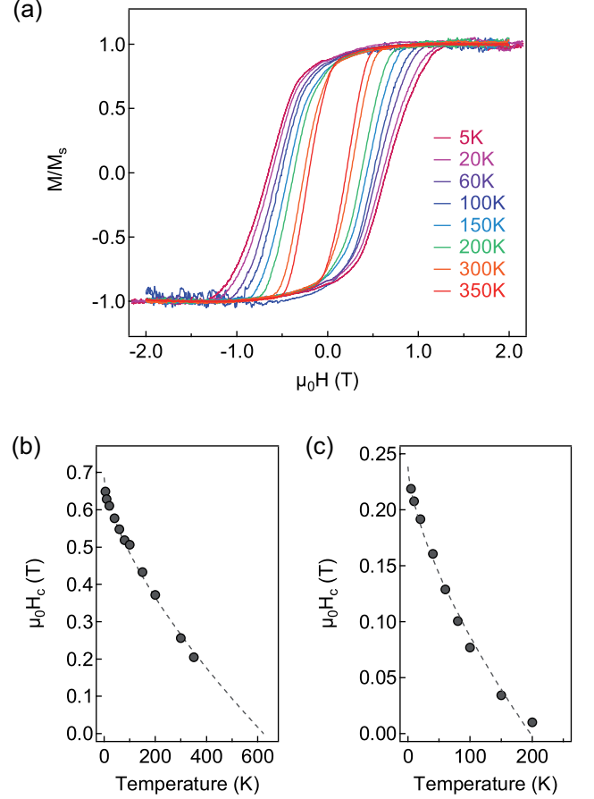
FIG. 8. (Color online) Thermal evolution of magnetic hysteresis cycles measured by VSM. (a) Cycles from 5 to 350 K of sample S78, with the applied field along the nanowire axis. (b) Thermal evolution of the coercive field \mu_0 H_c in sample S78 (dots). The line is a fit to Sharrock's formula (Eq.(2)), with T_b = 623 K. (c) Same as (b) for sample S18, with T_b = 197 K.
