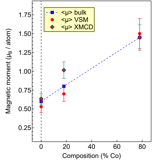
FIG. 10. Average magnetic moment \langle \mu \rangle for S00, S18 and S78 samples, as measured by VSM (disks) and XMCD using eq. (5) (diamonds). Squares: bulk values.
