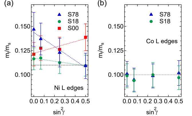
FIG. 11. m_l/m_s ratio, extracted from XMCD data by application of the sum rules, as a function of \sin^2 \gamma for samples S00, S18, and S78. (a) m_l/m_s ratio at Ni L_{2,3} edges, (b) m_l/m_s ratio at Co L_{2,3} edges. Black horizontal dashed line: bulk value.
