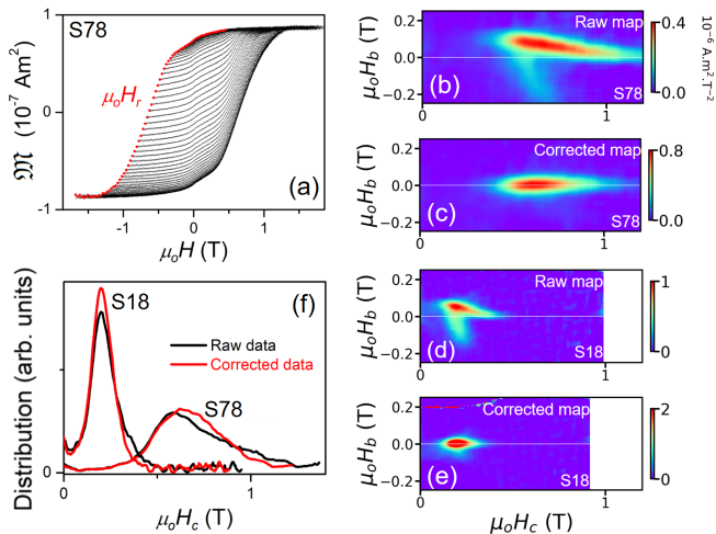
FIG. 7. (Color online) Coercive field distributions in samples S78 and S18 extracted from FORC measurements at 5 K with the field applied along the axis of the nanowires. (a) Reversal curves \mathfrak{M}(H_r, H) measured in sample S78, after saturation at 1.86 T prior to each reversal and with the reversal field \mu_0 H_r decreasing from 0.45 to -1.68 T in steps of -0.03 T (red dotted field positions). (b) Raw and (c) dipolar effect corrected FORC maps of sample S78. (d) Raw and (e) dipolar effect corrected FORC maps of sample S18. (f) Raw (black) and intrinsic (red/grey) coercive field distributions in samples S78 and S18, obtained by integrating the FORC maps along the \mu_0 H_c axis.
