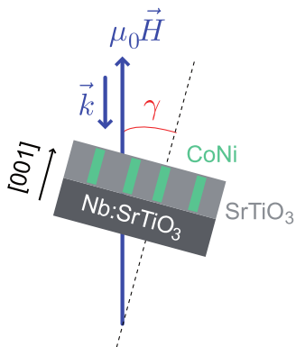
FIG. 2. (Color online) Geometry used for XMCD measurements. \vec{k} is the wavevector of soft x-rays, parallel to the applied magnetic field. \gamma is the angle between \vec{k} and the surface normal.
