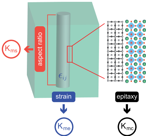
FIG. 1. (Color online) Control of magnetic anisotropies in vertically assembled nanostructures: the shape of embedded nanopillars determines the magnetostatic anisotropy K_{ms} , the strain leads to a magnetoelastic contribution K_{me} and the epitaxial relationship sets the easy and hard axes related to the magnetocrystalline anisotropy K_{mc} .
