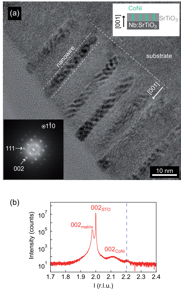
FIG. 3. (Color online) (a) High resolution TEM cross section of the S57 sample, acquired along the 1\bar{1}0 zone axis. Upper inset: schematics of the sample. Lower inset: Fourier transform of the image. (b) \theta - 2\theta scan of sample S78. The dashed vertical line indicates the position of the Bragg reflection of the unstrained bulk CoNi alloy.
