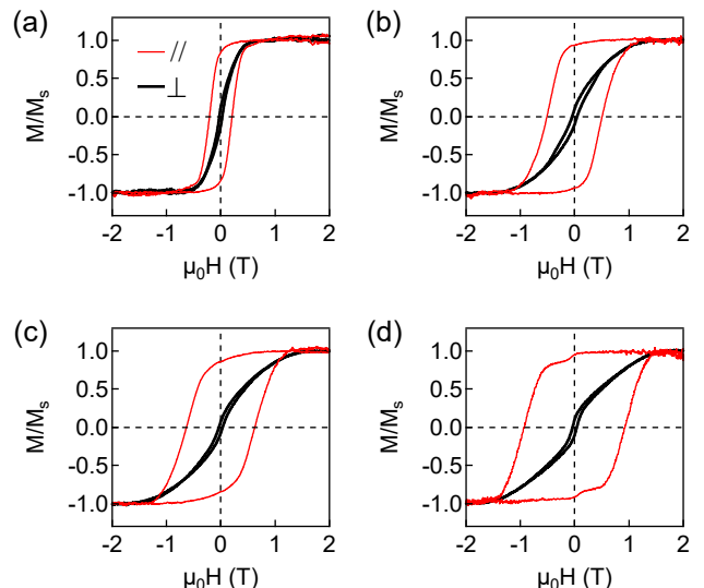
FIG. 4. Magnetic hysteresis cycles recorded at T=10 K with the applied magnetic field along the axis of the nanowires (thin line) and perpendicular to it (thick black line) for samples S18 (a), S57 (b), S78 (c), and S80 (d).
