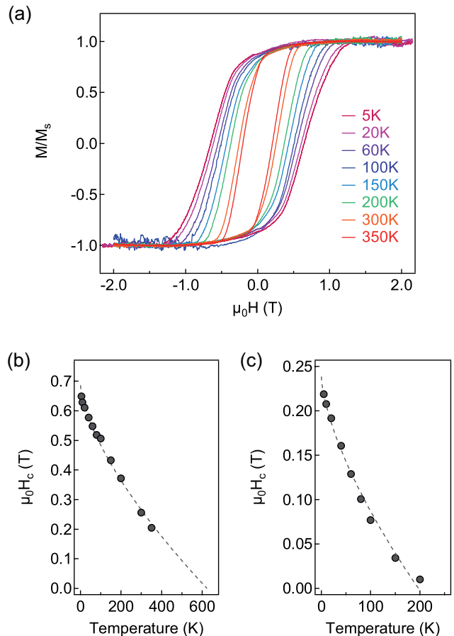
FIG. 8. (Color online) Thermal evolution of magnetic hysteresis cycles measured by VSM. (a) Cycles from 5 to 350 K of sample S78, with the applied field along the nanowire axis. (b) Thermal evolution of the coercive field \mu_0 H_c in sample S78 (dots). The line is a fit to Sharrock’s formula (Eq.(2)), with T_b = 623 K. (c) Same as (b) for sample S18, with T_b = 197 K.
