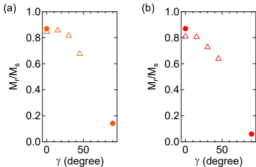
FIG. 6. Normalized remanence measured as a function of the angle \gamma between [001] and the applied magnetic field by XMCD at the Ni L_{2,3} edges at T=4.2 K (open triangles) and VSM at T=5 K (solid disks). (a) Results for S18 sample. (b) Results for S78 sample.
