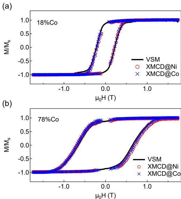
FIG. 5. Magnetic hysteresis cycles measured with the field applied along the axis of the nanowires ( \gamma=0 ) by XMCD at the Ni L_{2,3} edges (circles) and Co L_{2,3} edges (crosses) at T=4.2 K, and by VSM (line) at T=5 K. (a) Data for S18 sample. (b) Data for S78 sample.
