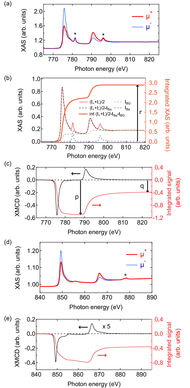
FIG. 9. XAS and XMCD spectra acquired at T=4.2 K and \gamma=0 at the Co and Ni L_{2,3} edges on sample S78. (a) XAS spectra for \mu^+ and \mu^- configurations at the Co L_{2,3} edges. The peaks marked by asterisks are due to Ba impurities in the SrTiO 3 matrix. (b) Averaged XAS spectrum (background corrected) and its integral after Ba contribution ( I_{Ba} ) and background ( I_{BG} ) removal. (c) XMCD at the Co L_{2,3} edges. Black line: spectrum, red (gray) line: integrated signal. Note that the spectral features related to Ba in XAS do not give rise to any significant dichroic signal. (d) XAS spectra for \mu^+ and \mu^- configurations at the Ni L_{2,3} edges. The peak marked by an asterisk is due to Ce impurities in the SrTiO 3 matrix. (e) XMCD at the Ni L_{2,3} edges. Black line: spectrum, red (gray) line: integrated signal.
