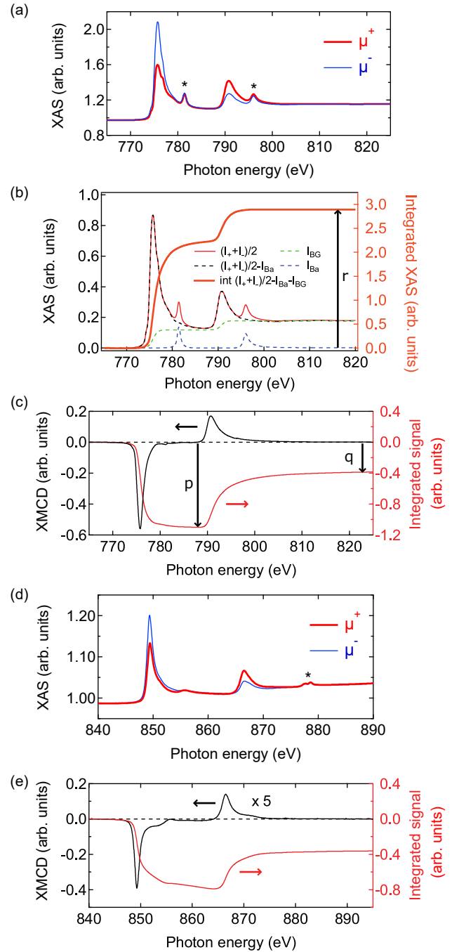
FIG. 9. XAS and XMCD spectra acquired at T=4.2 K and \gamma=0 at the Co and Ni L_{2,3} edges on sample S78. (a) XAS spectra for \mu^+ and \mu^- configurations at the Co L_{2,3} edges. The peaks marked by asterisks are due to Ba impurities in the SrTiO 3 matrix. (b) Averaged XAS spectrum (background corrected) and its integral after Ba contribution ( I_{Ba} ) and background ( I_{BG} ) removal. (c) XMCD at the Co L_{2,3} edges. Black line: spectrum, red (gray) line: integrated signal. Note that the spectral features related to Ba in XAS do not give rise to any significant dichroic signal. (d) XAS spectra for \mu^+ and \mu^- configurations at the Ni L_{2,3} edges. The peak marked by an asterisk is due to Ce impurities in the SrTiO 3 matrix. (e) XMCD at the Ni L_{2,3} edges. Black line: spectrum, red (gray) line: integrated signal.
