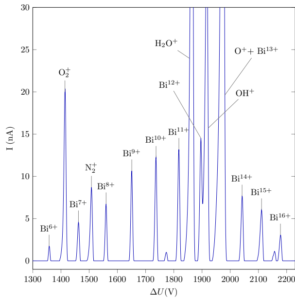
FIG. 2. Spectrum of a Bismuth beam measured at the entrance of the pulsing system. \Delta U corresponds to the voltage difference applied on the Wien filter electrodes.
