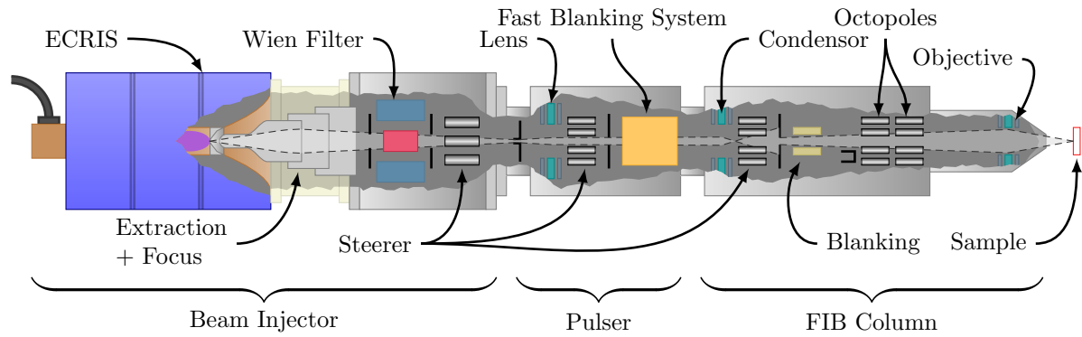
FIG. 1. Schematic of the EVOL FIB column.
