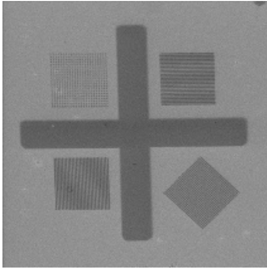
FIG. 5. SEM image (field of view of 250 \mu\text{m} ) of a milling made on an LSMO sample by O + ions at 20 keV with different patterns: matrix of dots on the top left, horizontal lines on the top right, vertical ones on the bottom left and oblique ones on the bottom right. The 200 \times 200 \mu\text{m} cross is engraved by Ar + ions at 20 keV.
