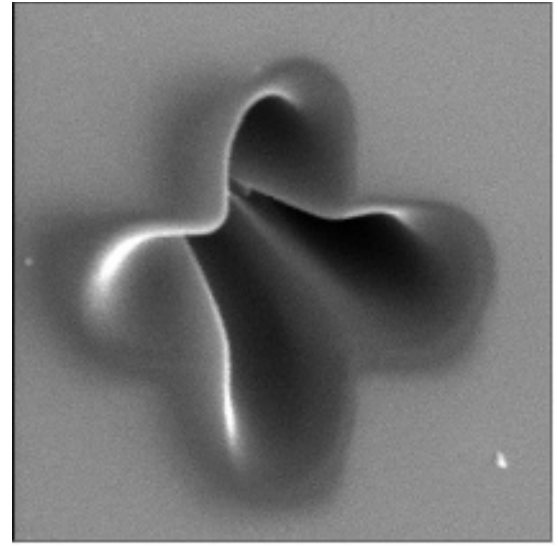
FIG. 6. SEM image (field of view of 9.2 \mu\text{m} ) of a cross obtained by Ar + ions milling at 20 keV on Si sample, with a fluence of 3.3 \times 10^{18} ions/cm.
