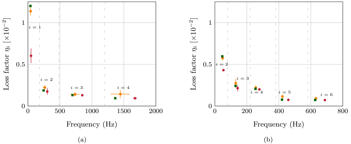
Figure 10: Measured loss factor for configurations ① in Figure 10(a) and ② in Figure 10(b) presented in this section: (—○) the experimental non-perforated plate, (—○) the experimental MPP, (—■) the theoretical MPP. Each loss factor is determined for the i th mode that refers to the three colours. The damping is optimized to reach a maximum value at f_i \approx f_c with i = 1 in Figure 10(a), i = 2 in Figure 10(b). In Figure 10(b), only modes in the domain of sensor's validity are represented.
