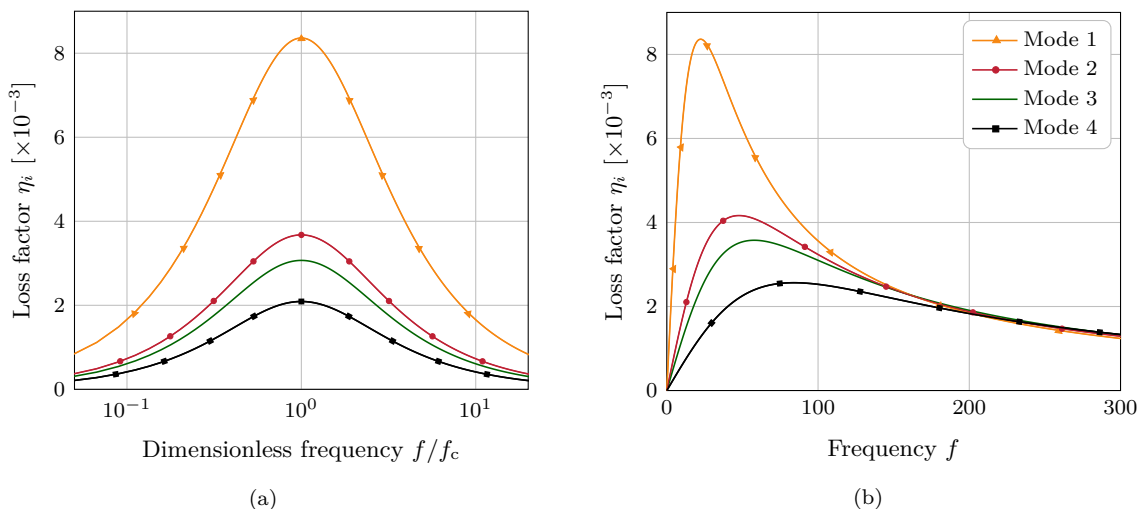
Figure 5: Loss factor given in Equation (47) for a simply-supported MPP of dimensions 490 mm \times 570 mm \times 1 mm (see Table 1) as function of frequency. In Figure 5(a) the diameter is fixed and f_c is a constant. The diameter is chosen to maximize the damping on f_1 , we therefore have f_1 = f_c . In Figure 5(b) the diameter is different for each mode and is chosen to maximize the damping in each mode. We therefore have f_i = f_c .
