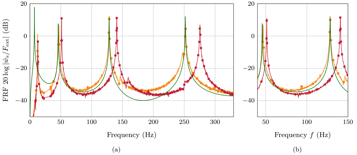
Figure 9: Mobility of various clamped-free plate: (—■) experimental non-perforated plate, (—○) experimental MPP ②, (—) theoretical MPP ②. For theoretical and measured MPP ②, the damping is optimized to be maximum for the second natural mode, f_2 , and not for f_1 as in Figure 8. The Figure 9(a) corresponds to the frequency response for the first four modes while the Figure 9(b) is a zoom on the resonance mode f_2 and f_3 . In order to respect the domain of sensor's validity, the first natural mode, which occurs at f_1 \approx 8 Hz is not considered in the frequency response.
