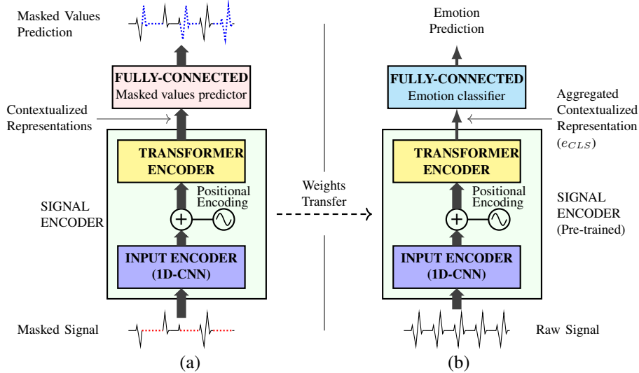
Figure 1: Our approach with self supervised learning based on a Transformer (a) and fine-tuning strategy for learning the final emotion predictor (b).
