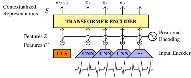
Figure 2: Our Transformer-based signal encoder that produces contextualized representations. The aggregated representation e_{CLS} is used for classification.
