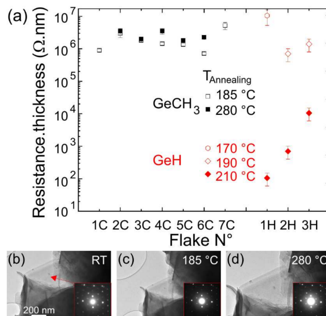
Figure 5. (a) Comparison of the product of the four-point resistances to the crystallite thickness for \text{GeCH}_3 (C) microcrystallites and H-passivated (H) flakes, measured as a function of the annealing temperature. The spacing between the electrodes or the tips varies in a range extending from 0.5 to 3.0 \mu\text{m} . The data for the H-passivated flakes were deduced from the experimental results published in Refs. [9,18]. (b–d) TEM images and SAED patterns of the thin edge of a microcrystallite collected at room temperature (RT), 185 ^{\circ}\text{C} and 280 ^{\circ}\text{C} , respectively.
