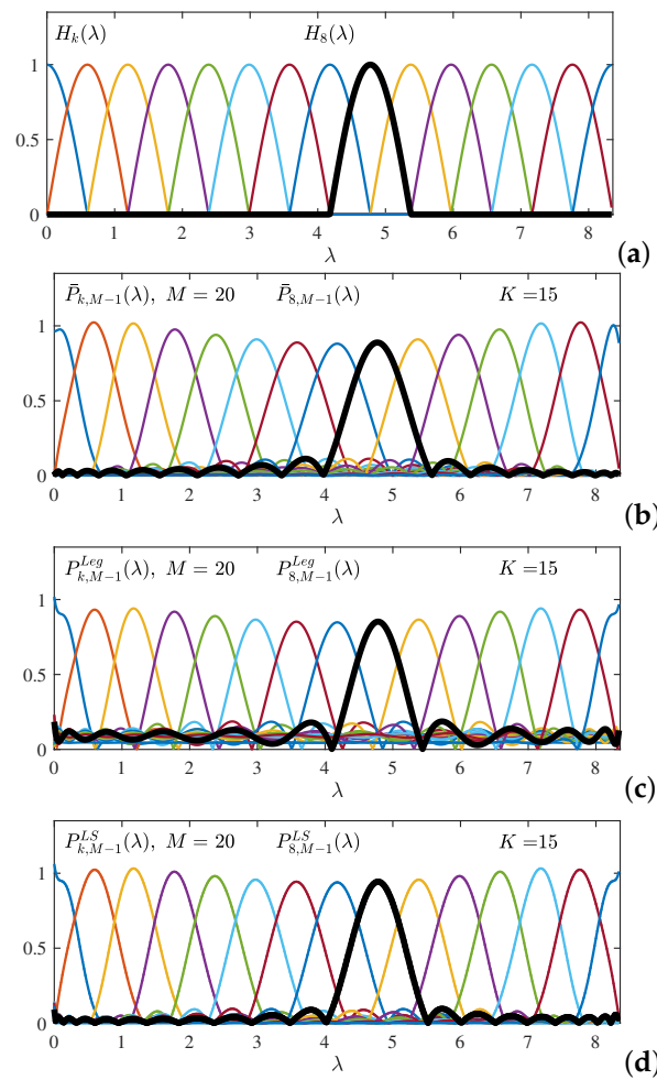
Figure 15. Spectral bandpass transfer functions used for calculation of the LGFT and their polynomial approximations. (a) Spectral functions of the Hann form with K = 15 . (b) Approximation of spectral transfer functions based on Chebyshev polynomial with M = 20 . (c) Legendre-polynomial-based approximations of spectral transfer functions with M = 20 . (d) Least squares approximation of spectral transfer functions with M = 20 . For convenience, function H_8(\lambda) is designated with a thick black line on each panel.
