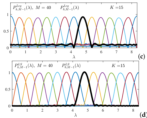
Figure 16. Spectral bandpass transfer functions used for calculation of the LGFT and their polynomial approximations. (a) Spectral functions of the Hann form with K = 15 . (b) Approximation of spectral transfer functions based on Chebyshev polynomial with M = 40 . (c) Legendre-polynomial-based approximations of spectral transfer functions with M = 40 . (d) Least squares approximation of spectral transfer functions with M = 40 . For convenience, function H_8(\lambda) is designated with a thick black line on each panel.
