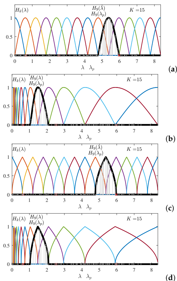
Figure 12. Transfer functions formed using the Hann window (a,b) and the Bartlett window (c,d) square root so that the reconstruction condition \sum_{k=0}^{K-1} H_k^2(\lambda_p) = 1 is satisfied, for a uniform splitting (a,c) of the spectral domain and a wavelet-like splitting (b,d).
