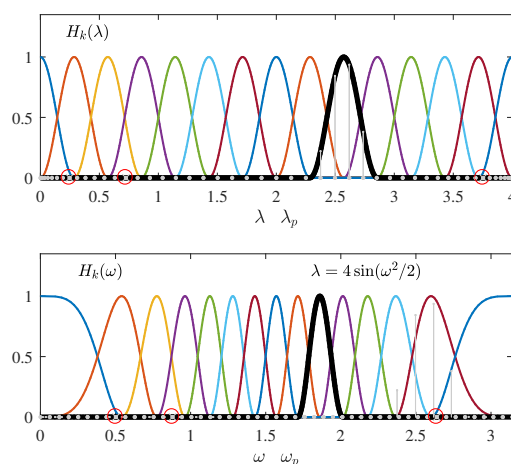
Figure 8. Transfer functions in the spectral eigenvalue and frequency domains for classical analysis: (top) The eigenvalue spectral domain transfer functions H_k(\lambda_p) , p = 1, 2, \dots, N , k = 0, 1, \dots, K - 1 , for K = 15 and 0 \leq \lambda \leq \lambda_{\max} = 4 . (down) The frequency spectral domain transfer functions H_k(\omega_p) , p = 1, 2, \dots, N , k = 0, 1, \dots, K - 1 , for K = 15 and 0 \leq \omega \leq \pi . Horizontal axis represents the continuous variable \lambda and discrete values \lambda_p , p = 1, 2, \dots, N , corresponding to the eigenvalues and denoted by gray dots along the axis. The same notation is used for frequency \omega and its discrete values \omega_p that correspond to \lambda_p .
