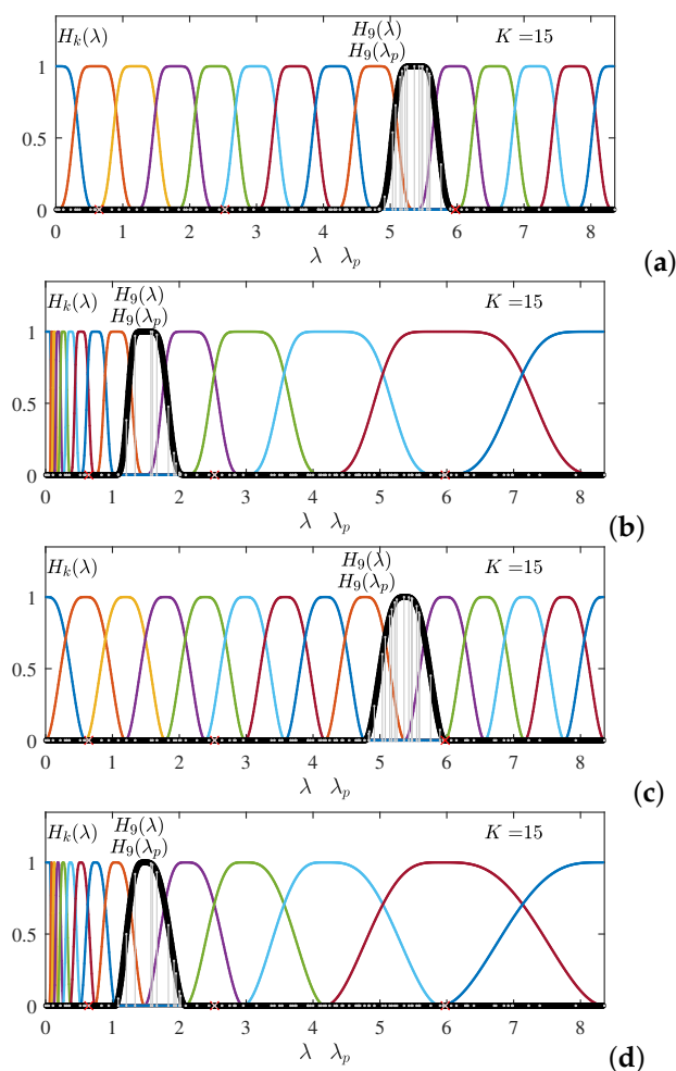
Figure 13. Transfer functions formed using the Hann window (a,b) and the Bartlett window square root with modified argument (c,d), using the argument x mapping v_x(x) = x^4(35 - 84x + 70x^2 - 20x^3) . The WOLA reconstruction condition \sum_{k=0}^{K-1} H_k^2(\lambda_p) = 1 is satisfied.
