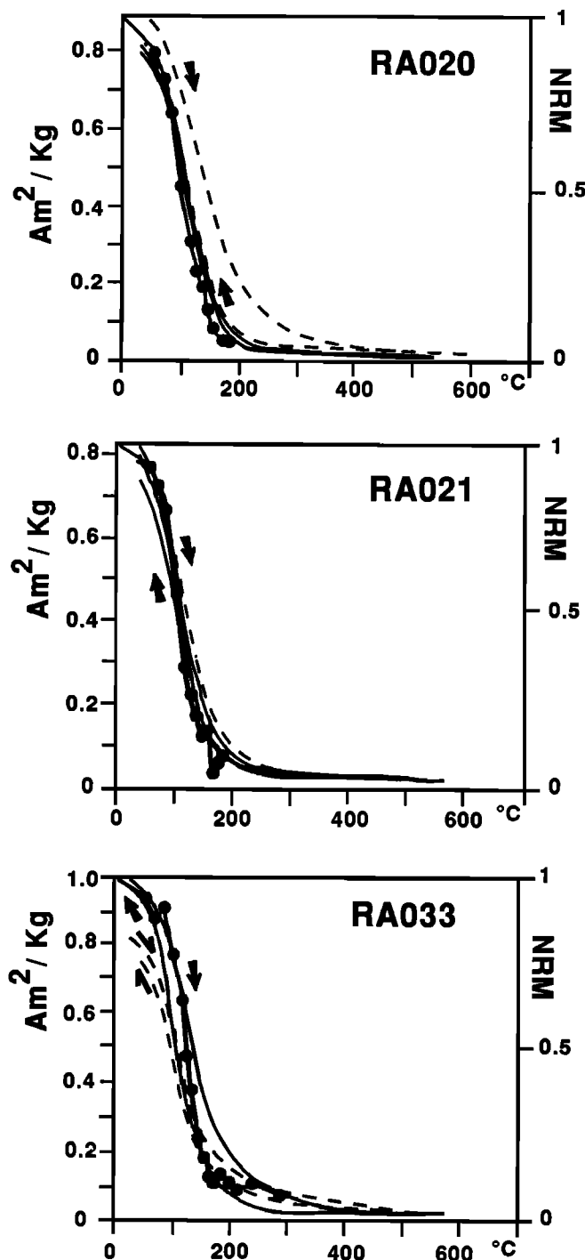
Fig. 20. Comparison of the NRM demagnetization (solid circles) with J_s - T experiments. Solid curves (dashed curves) correspond to Curie curves before (after) the paleointensity experiment. Very few variations in the Curie temperature are observed.
