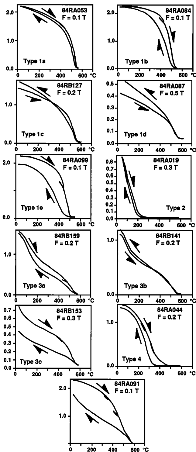
Fig. 4. Examples of Curie experiments performed in vacuum showing the different types of behavior. The value of the applied field ( F , in tesla) is indicated for each experiment. Heating and cooling curves are shown by arrows. The unit of the magnetic moment ( J_S ) is given in A\ m^2\ Kg^{-1} .
