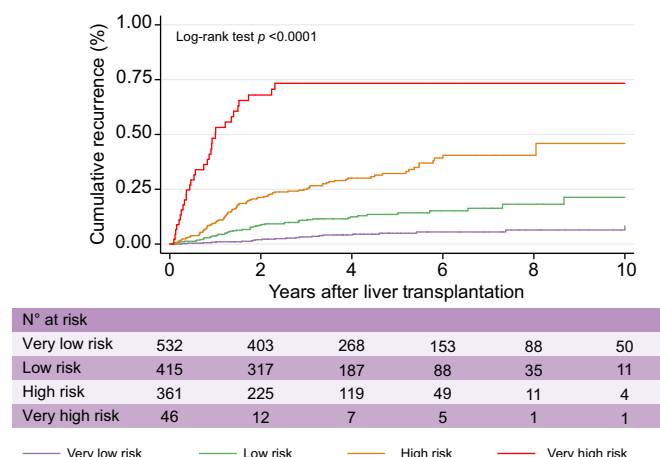
Fig. 1. Cumulative recurrence curves in the test cohort according to R3-AFP score categories. R3-AFP, recurrence risk reassessment–alpha-foetoprotein.
